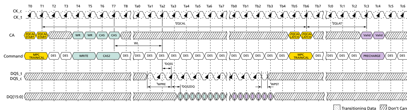
Figure 139: ZQCAL Timing
