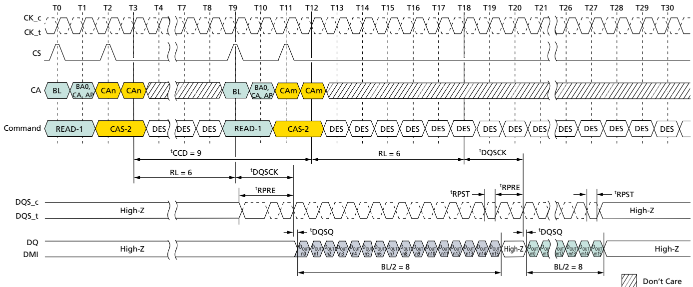
Figure 45: Consecutive READ: t_{CCD} = \text{MIN} + 1 , Preamble = Toggle, 0.5n\text{CK} Postamble
