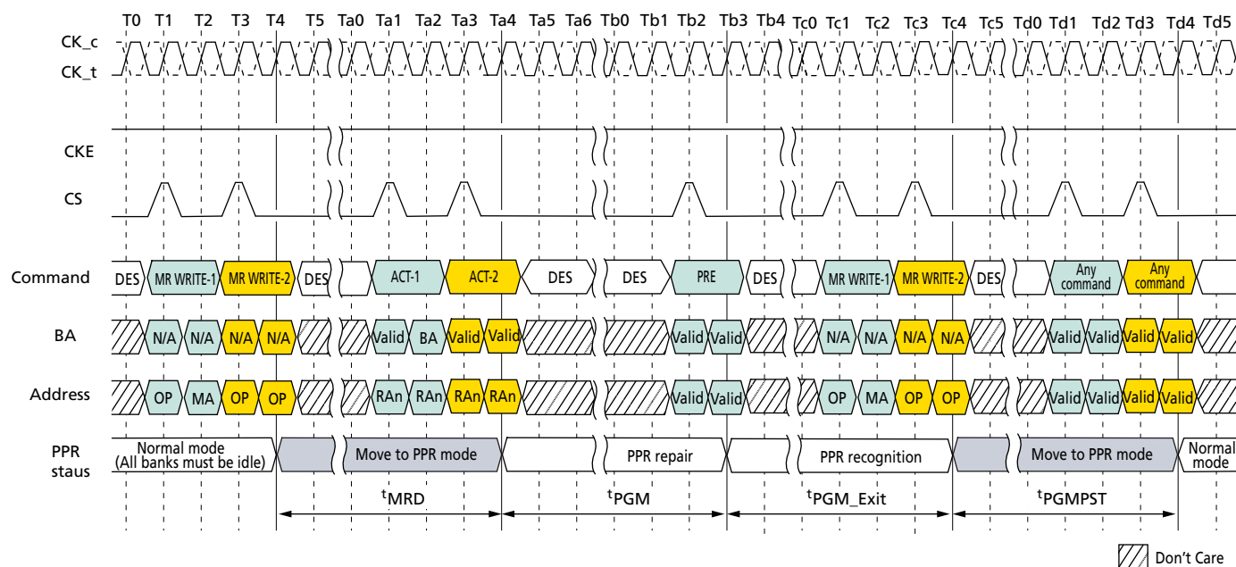
Figure 149: Post-Package Repair Timing
