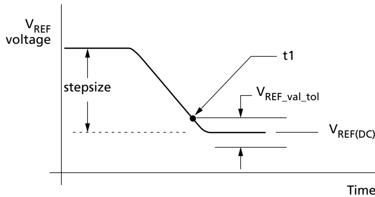
Figure 107: V REF(CA) Full Step from V REF,min to V REF,max
