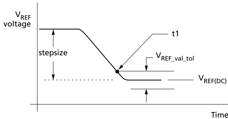
Figure 114: V REF (DQ) Full Step from V REF,min to V REF,max
