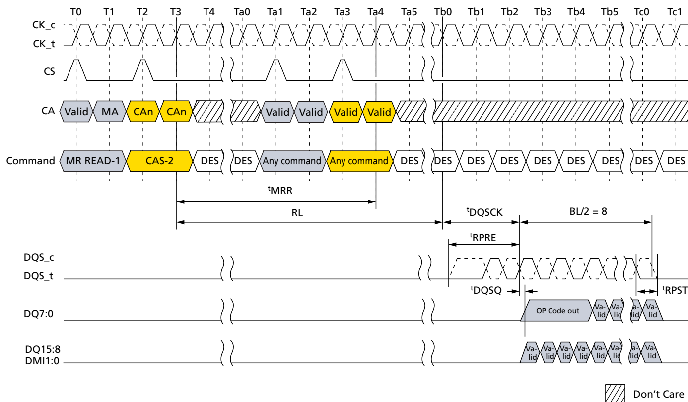
Figure 95: MODE REGISTER READ Operation
