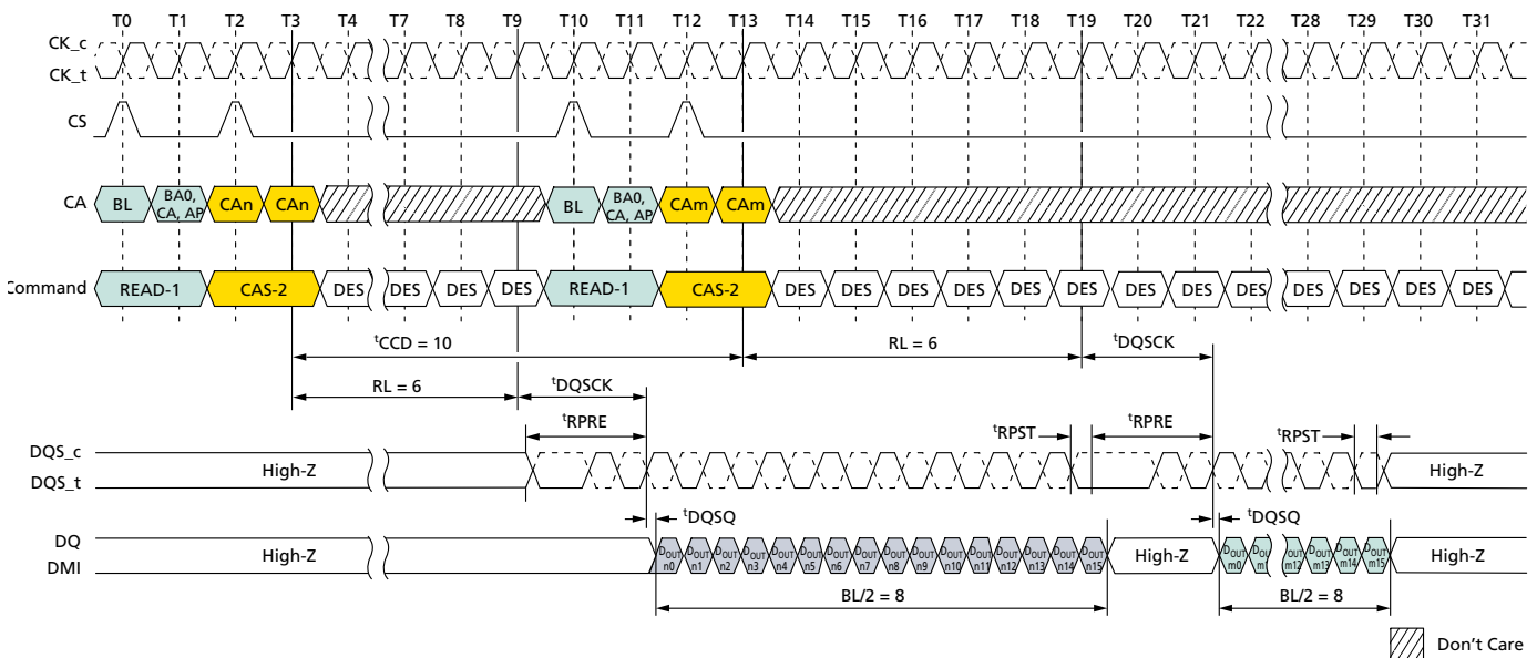
Figure 49: Consecutive READ: t_{CCD} = \text{MIN} + 2 , Preamble = Toggle, 0.5n\text{CK} Postamble
