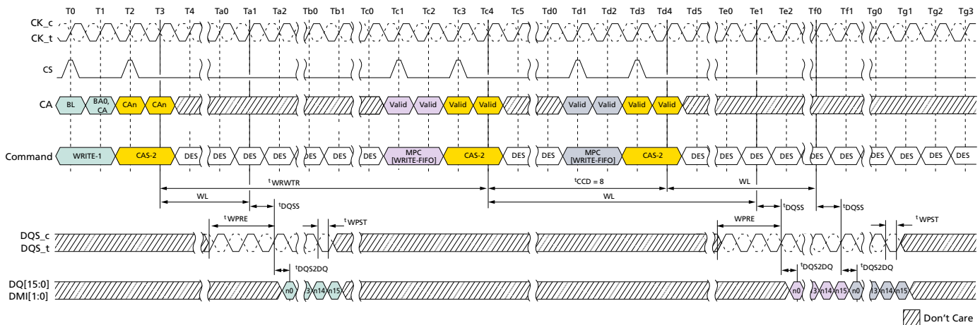
Figure 124: WRITE-FIFO – t_{WPRE} = 2nCK , t_{WPST} = 0.5nCK
