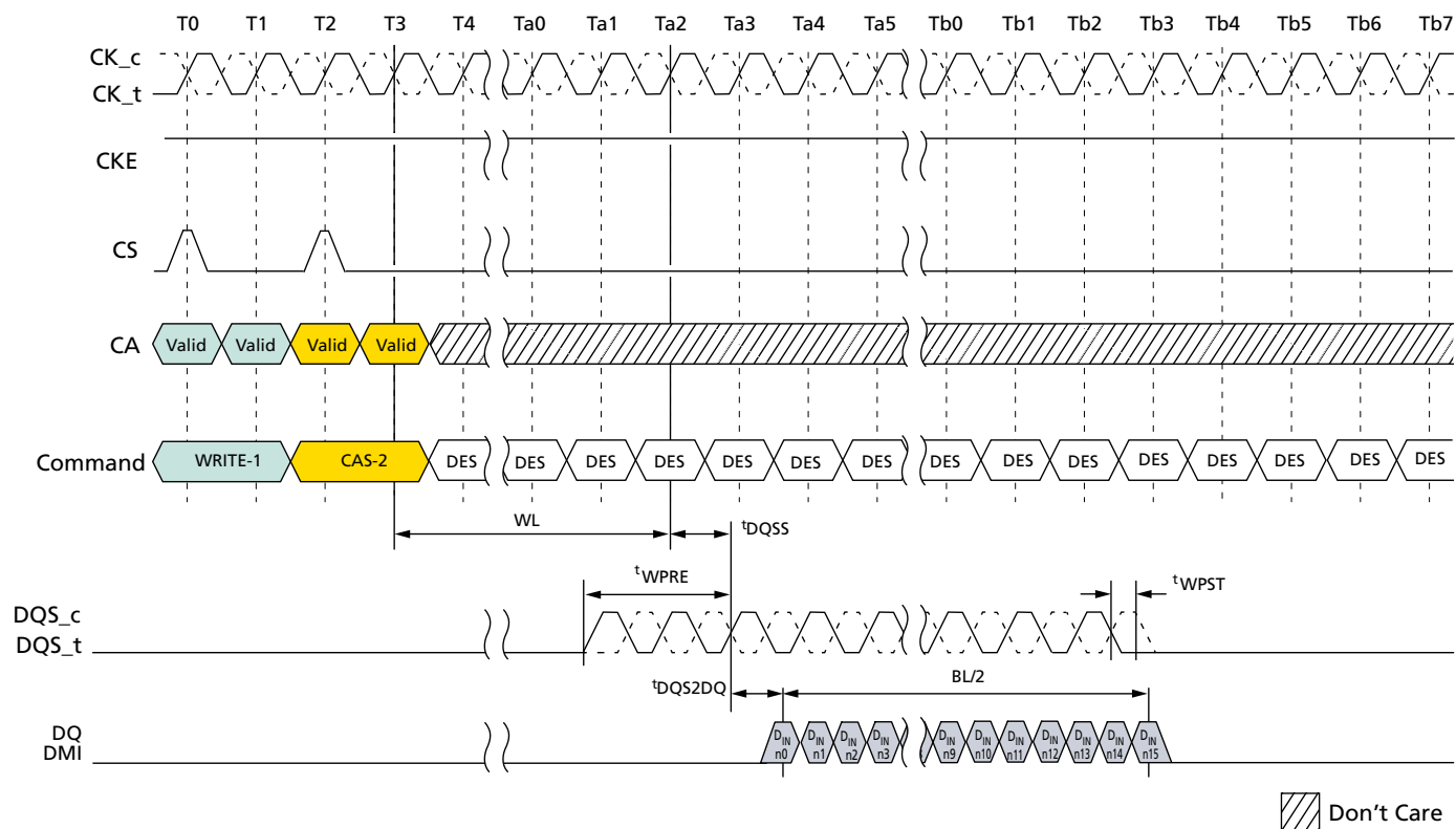
Figure 20: DQS Write Preamble and Postamble – 0.5nCK Postamble
