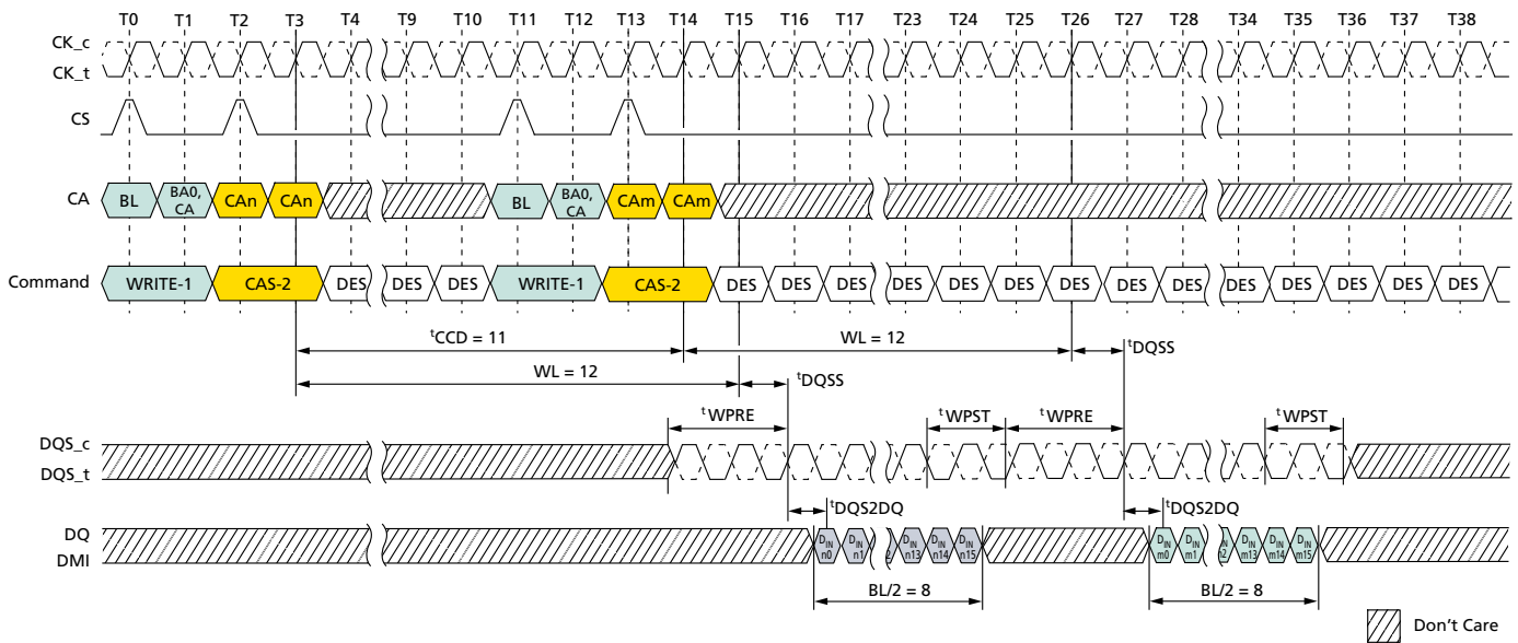
Figure 64: Consecutive WRITE: t_{CCD} = \text{MIN} + 3, 1.5n\text{CK} Postamble
