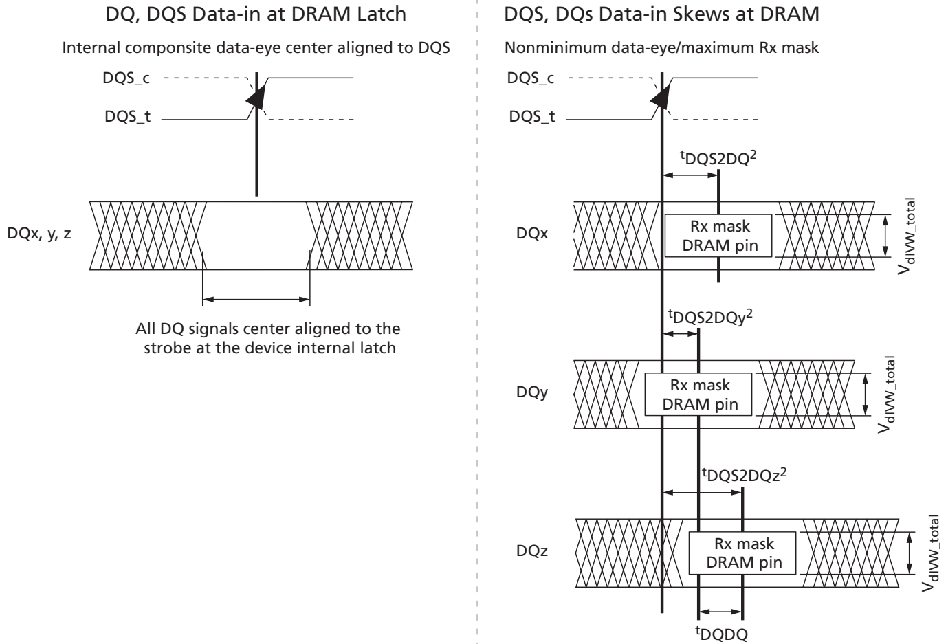
Figure 179: DQ-to-DQS t_{DQS2DQ} and t_{DQDQ}
