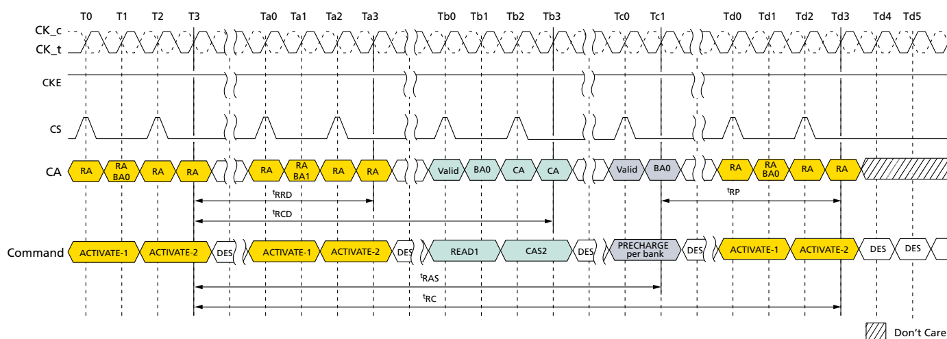
Figure 16: ACTIVATE Command
