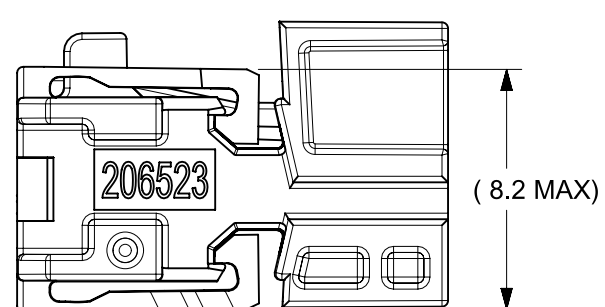
HINGE CLOSED
