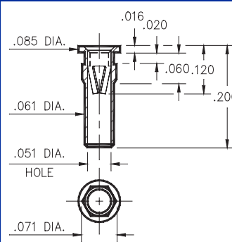
9293-0-15-XX-06-XX-10-0 Hex press-fit in .067 plated thru hole
