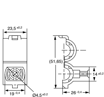
2, 3, 4 Contacts Part no. 029-8514-001
