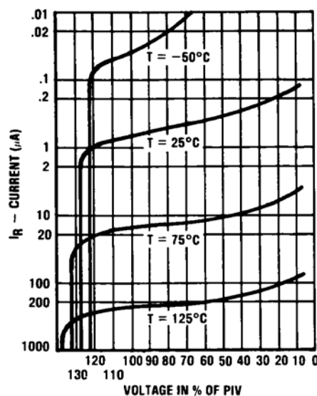
FIGURE 2 TYPICAL REVERSE CURRENT vs. VOLTAGE
