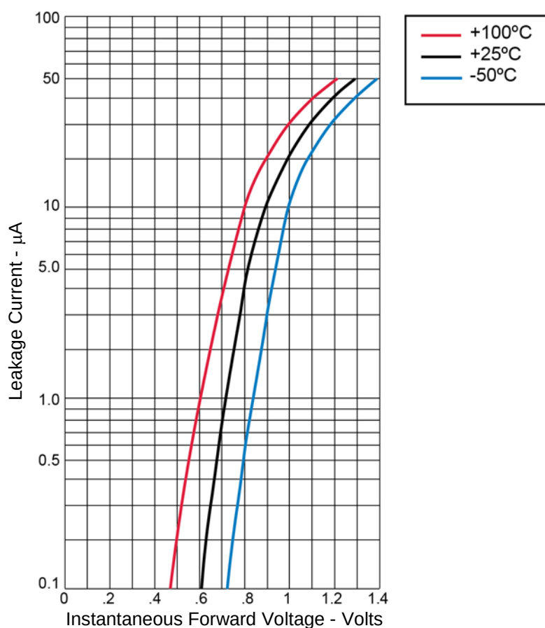
FIGURE 4 Typical Forward Characteristics – Per Leg 801 Series
