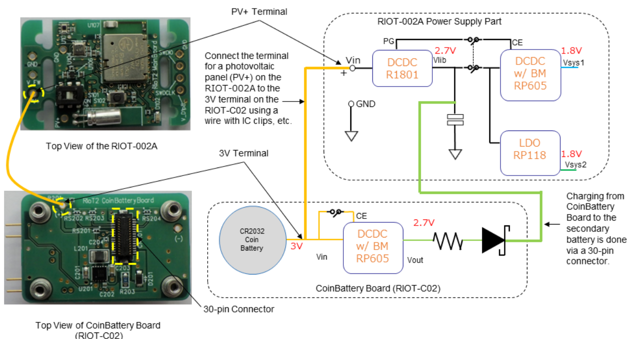
Figure 3. Connection between 3V Terminal of Coin Battery Board and PV+ Terminal of RIOT-002A
