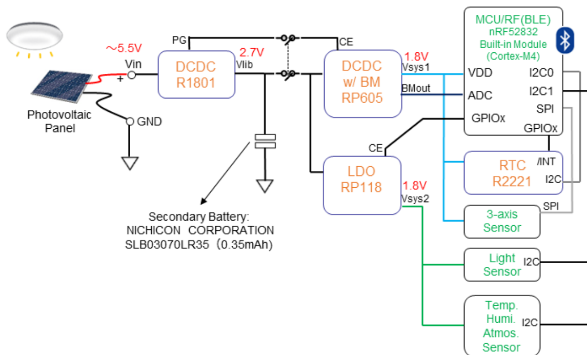
Figure 2. Block Diagram of RIOT-002A
