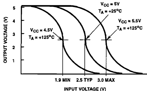
FIGURE 7. ACTUAL MIN/MAX AND TYPICAL SWITCHING CHARACTERISTICS OF THE HCU04 UNBUFFERED HEX INVERTER
