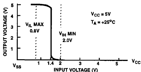
FIGURE 4. TYPICAL SWITCHING CHARACTERISTICS OF HARRIS HCT SERIES TYPES
