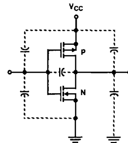
FIGURE 1. PARASITIC CAPACITANCES IN A CMOS INVERTER
