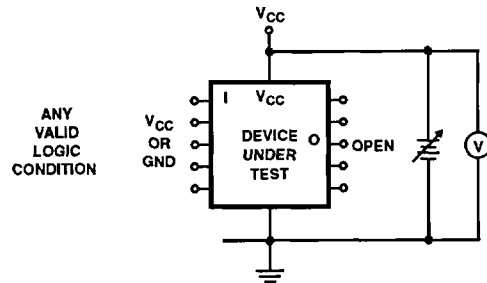
FIGURE 18. TEST SET-UP FOR V_{CC} OVER-VOLTAGE LATCH TRIGGER
