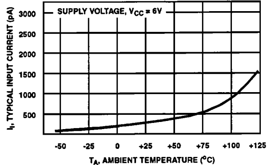
FIGURE 8. TYPICAL HC/HCT INPUT CURRENT vs TEMPERATURE
