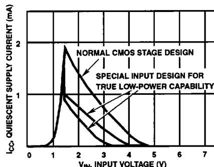
FIGURE 30. I_{CC} vs V_{IN} FOR HCT TYPES
