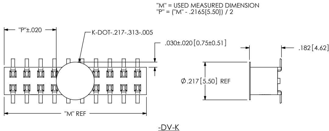
FIG 6 -K: POLYIMIDE FILM PAD ONLY AVAILABLE ON -SV & -DV (MMS-140-02-XXX-XV-K SHOWN) (DIFFERENT AS SHOWN, OTHERWISE SAME AS FIG 1)
