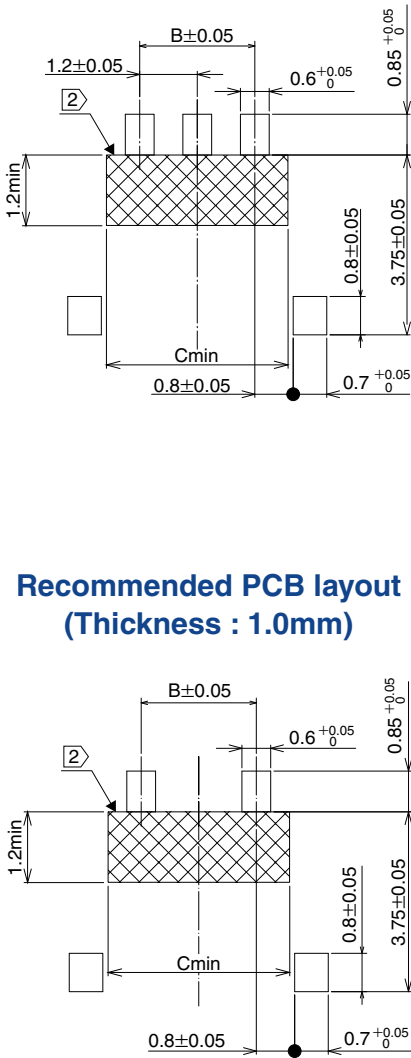
Recommended PCB layout (Thickness : 1.0mm)
