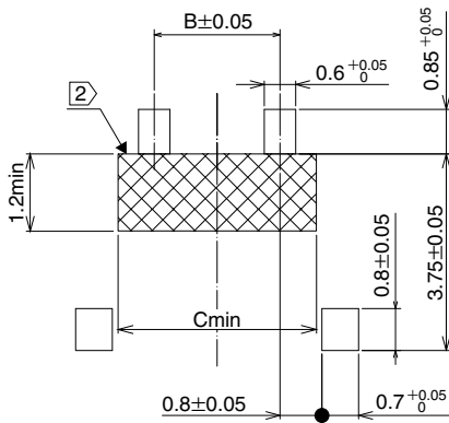
Recommended PCB layout (Thickness : 1.0mm)
