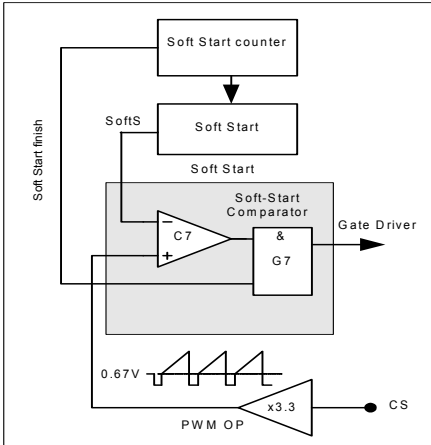
Figure 9 Soft Start
