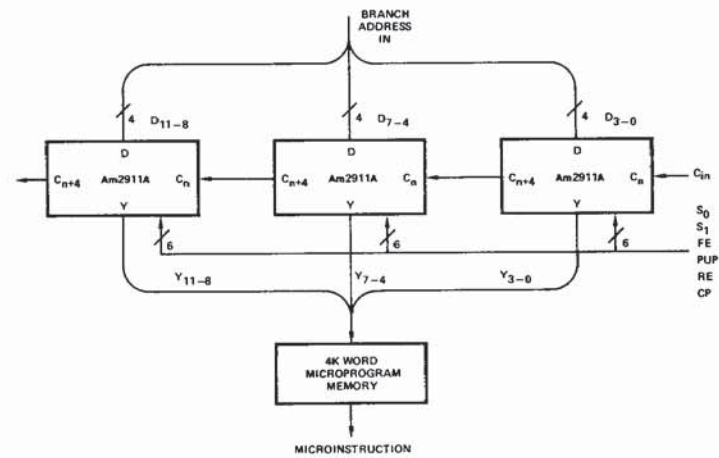
Figure 8. 12-Bit Sequencer
