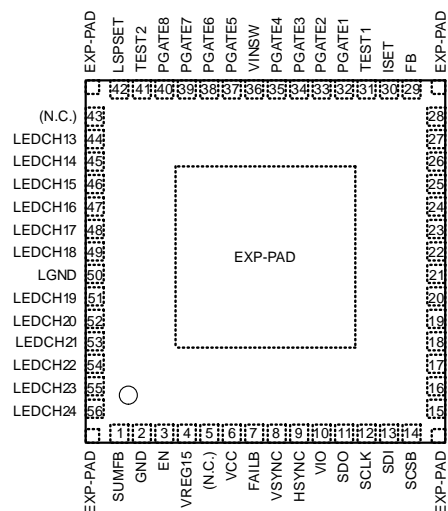
VQFN56FCV080 (TOP VIEW)
