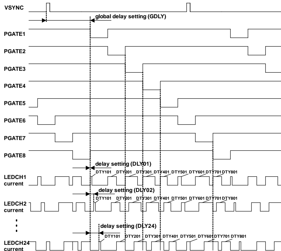
Figure 2. Delay Control
