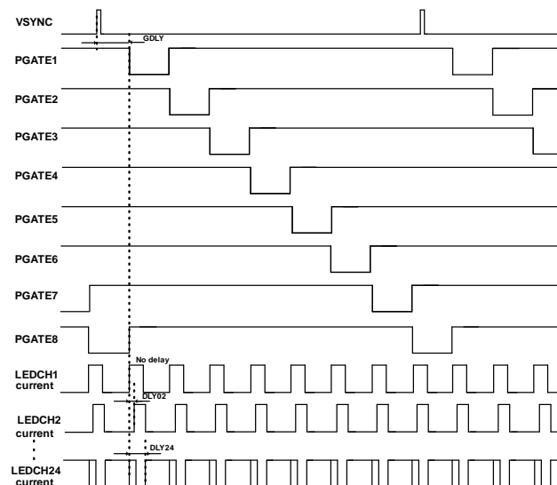
Figure 24. Dimming Mode
