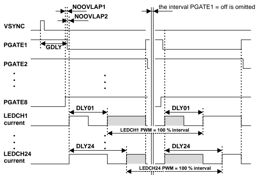
Figure 26. PWM delay setting
