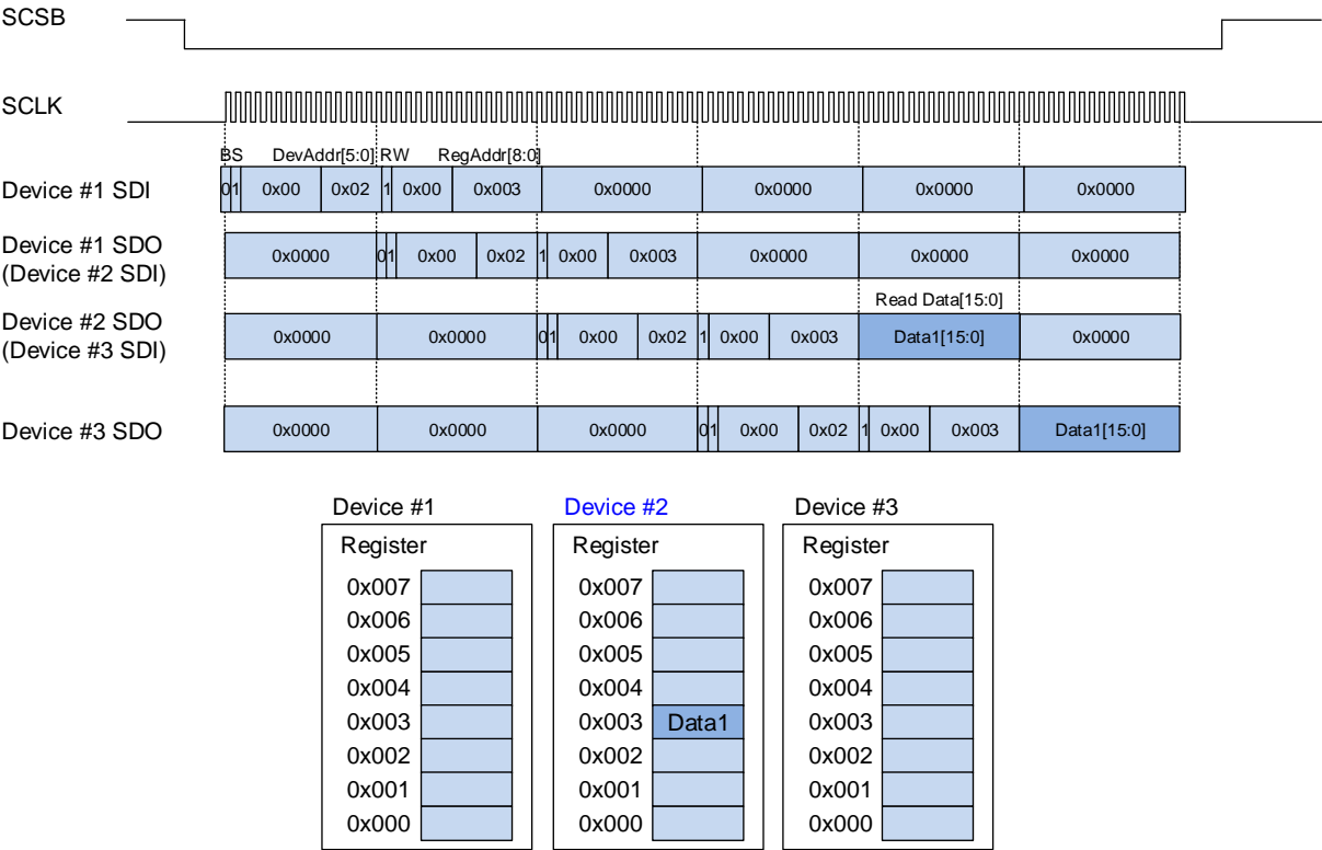
Figure 18. SPI Protocol for 1 Address Read from Device #2
