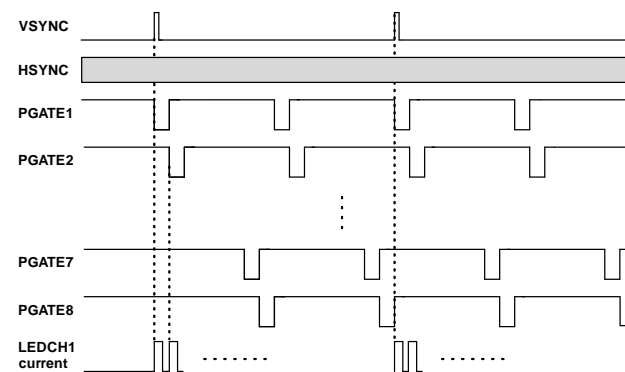
Figure 25. PWMFREQ vs LEDCHn output
