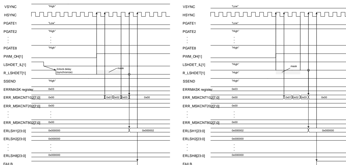
Figure 33. LED Short Detection and Release
