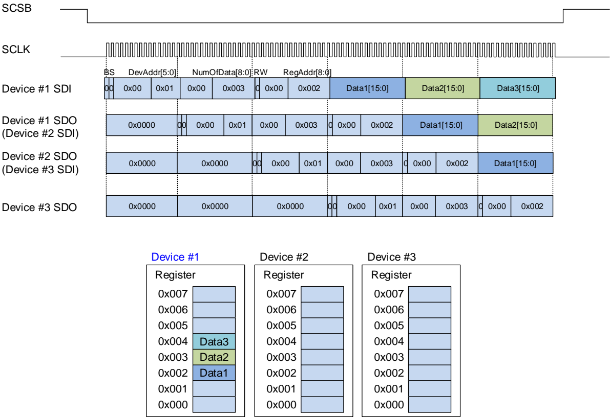
Figure 13. SPI Protocol for N Address Write to Device #1
