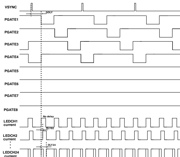
4 Line Gate Controller (MULSEL[1:0] = 0x1)
