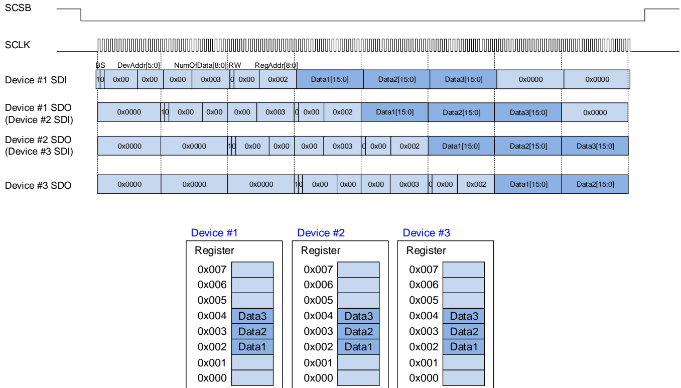
Figure 17. SPI Protocol for N Address Same Data Write to All Devices
