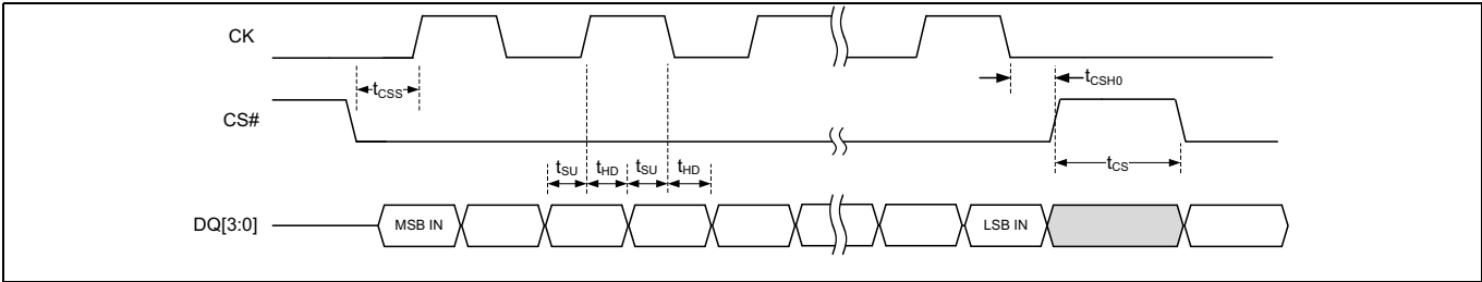
Figure 83 Quad and QPI DDR input timing
