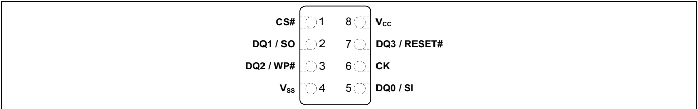
Figure 3 8-connector package (WSO6 6 x 8), top view
