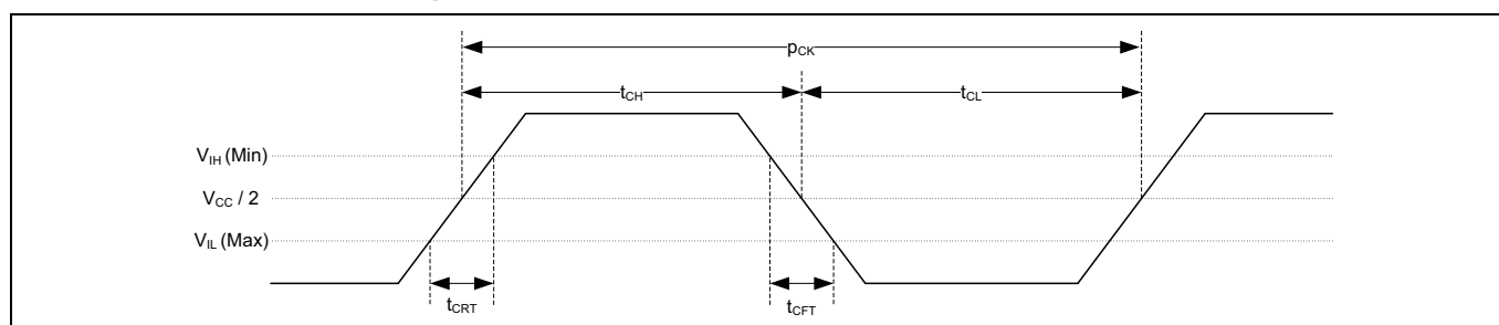
Figure 78 Clock timing
