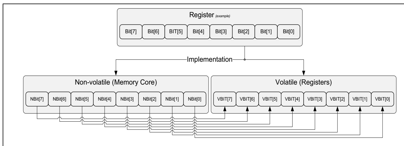
Figure 68 Register structure
