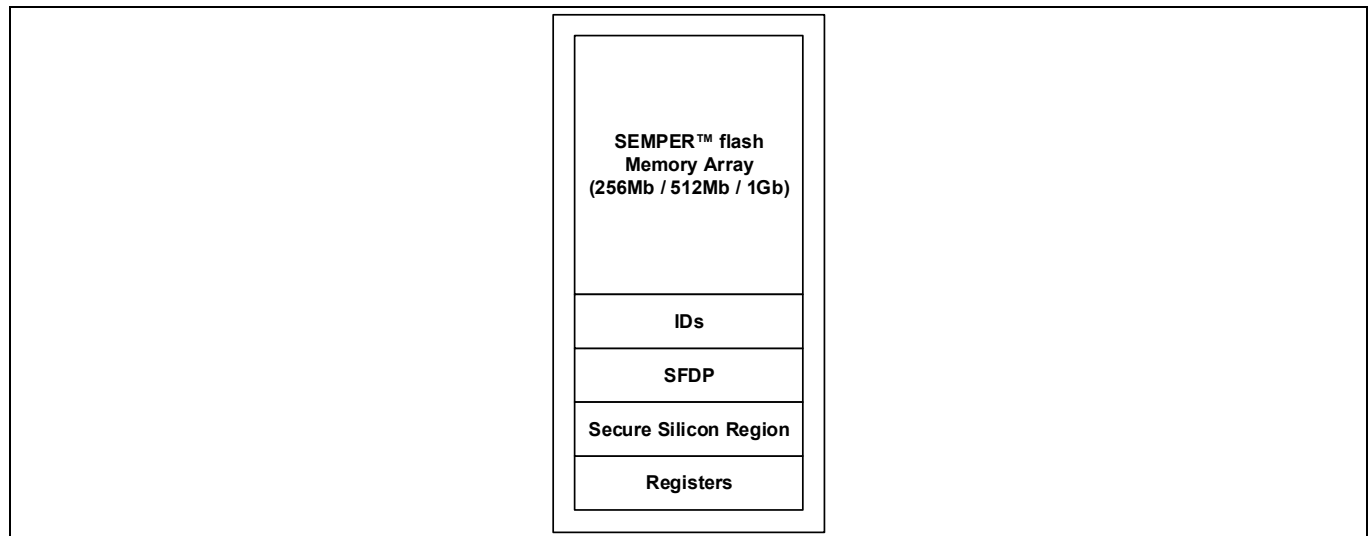
Figure 39 HL-T/HS-T address space map overview
