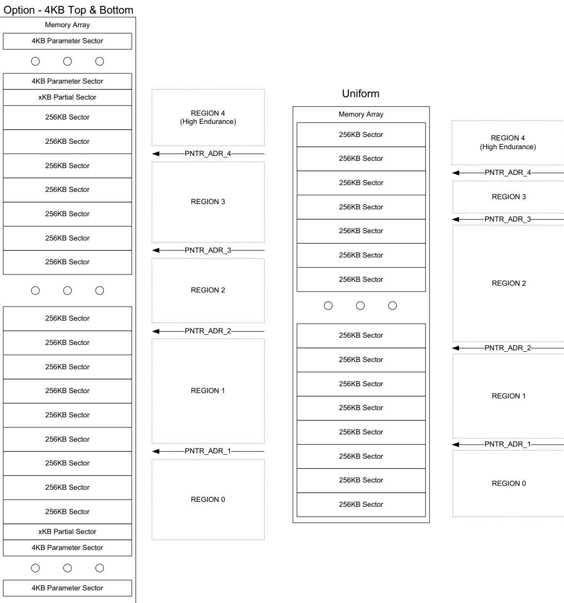
Figure 42 Infineon Endurance Flex architecture overview (Continued)
