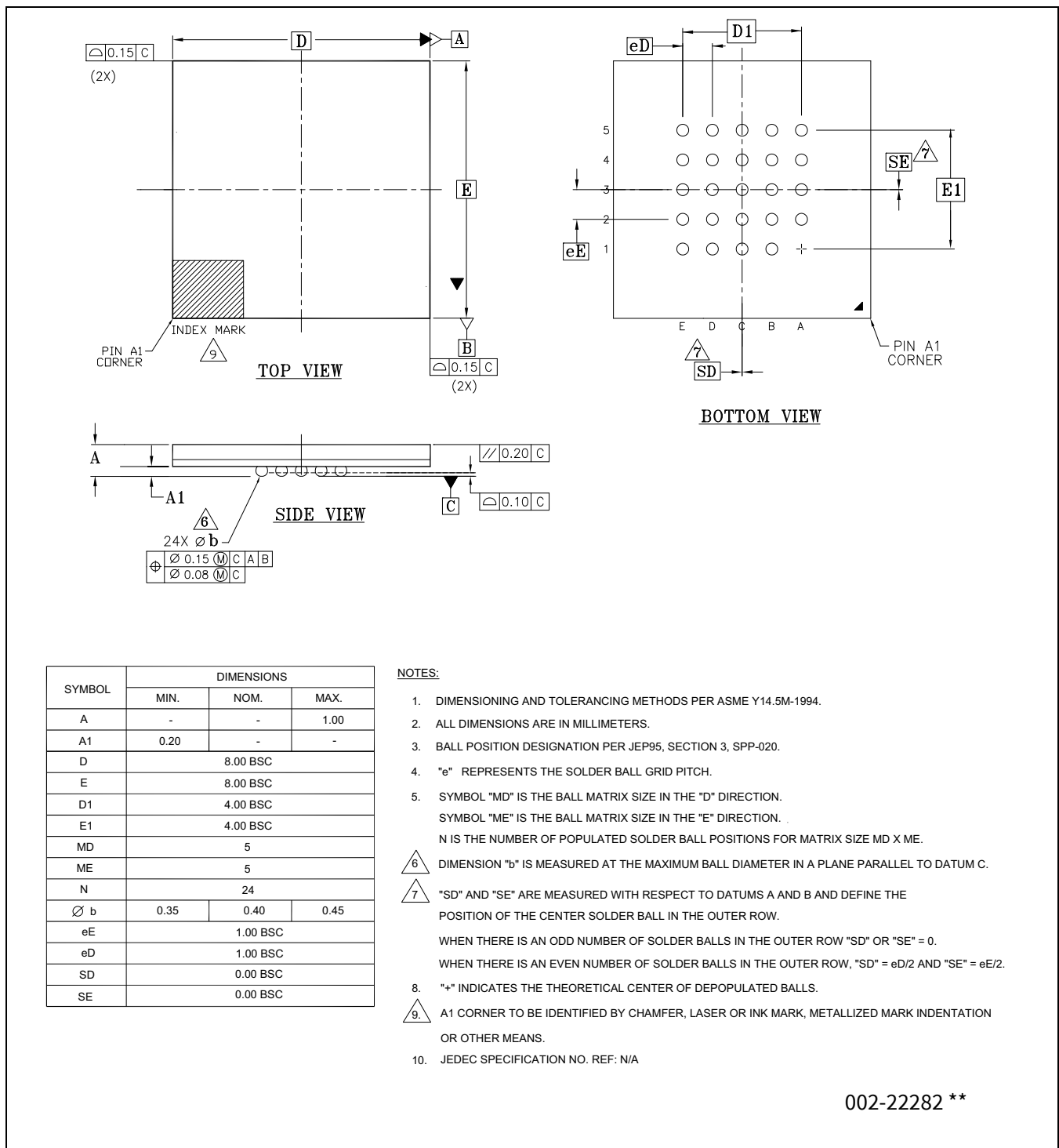
Figure 86 24-ball BGA (8.0 x 8.0 x 1.0 mm) package outline (PG-BGA-24), 002-22282
