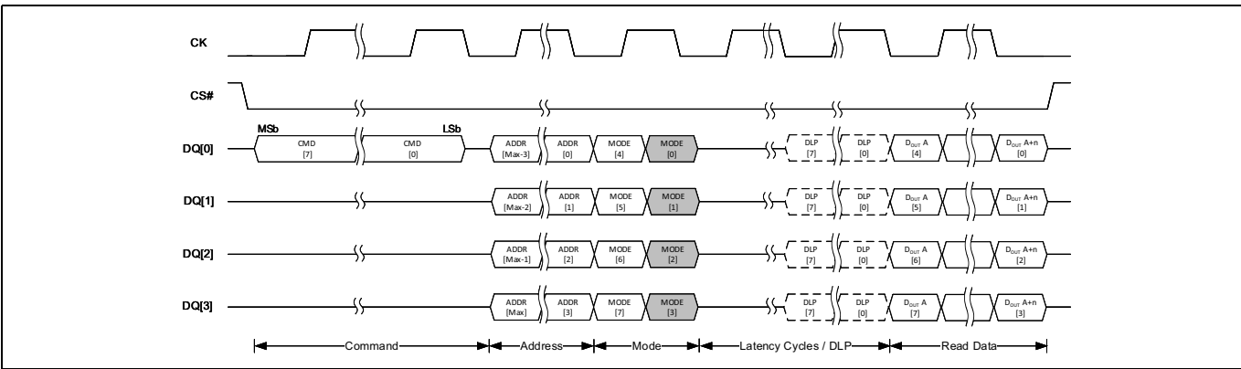
Figure 18 QOR SDR read transaction with command, address, and mode input (output latency)
