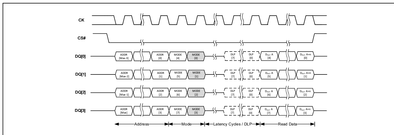
Figure 20 QIO SDR continuous read transaction with address and mode input (output latency) [5]
