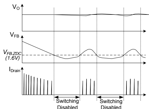
Figure 31. Burst-Mode Operation
