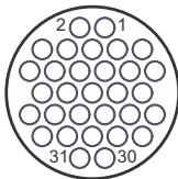
Shell Size 17 31 Contacts
