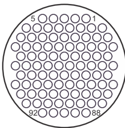
Shell Size 25 92 Contacts
