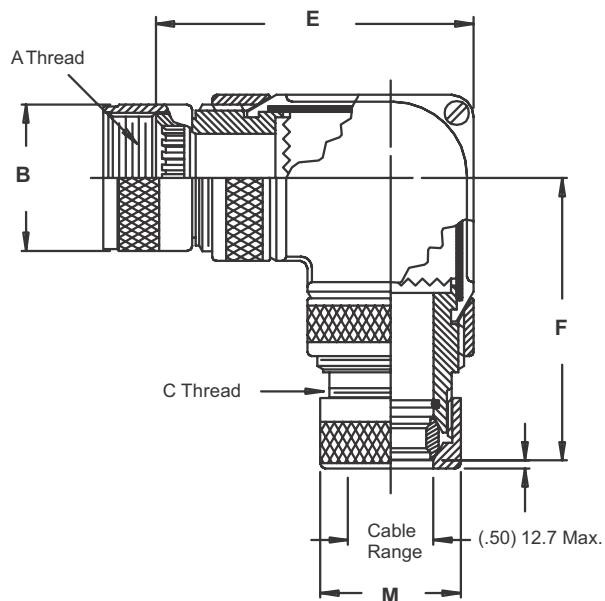
Style A- EMI/Non-Environmental (Plain Conduit)
