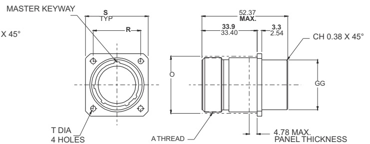
FIGURE 2 Long, 52.37 max length
