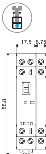
Type 22.32 + 022.33/022.35 Box clamp
