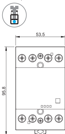
Types 22.44/22.64 Box clamp
