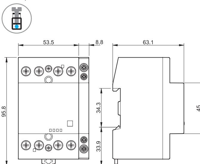
Types 22.44/22.64 + 022.63/022.65 Box clamp
