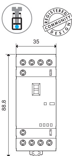
Type 22.34 Box clamp
