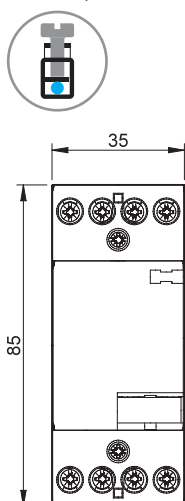
Types 22.74 Box clamp
