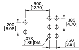
P.C.MOUNTING
