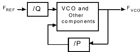
Figure 1. Simplified PLL
