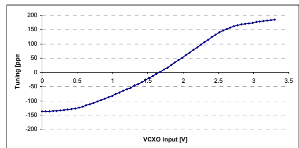
Figure 2. VCXO Profile
