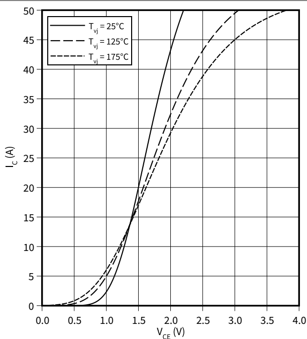
output characteristic (typical), IGBT-Chopper I_C = f(V_{CE}) V_{GE} = 15 V
