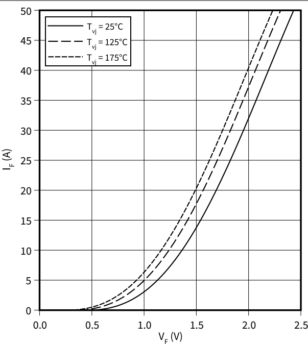
forward characteristic (typical), Diode, Chopper I_F = f(V_F)
