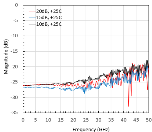
Output RL 20 dB, 15 dB, and 10 dB Attenuation
