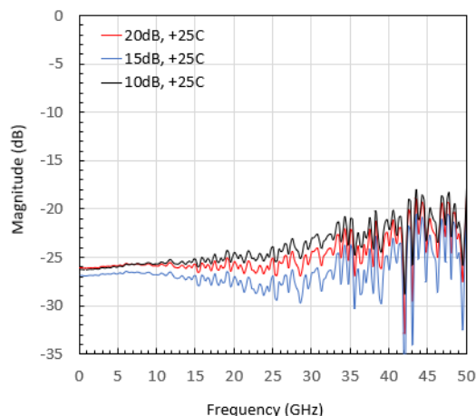
Input RL 20 dB, 15 dB, and 10 dB Attenuation
