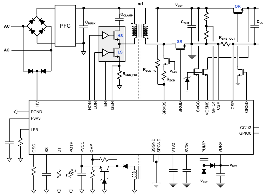
Figure 4. Typical configuration
