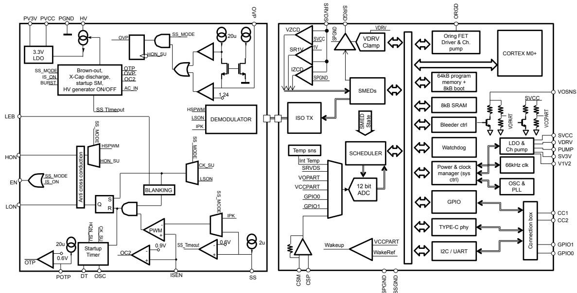
Figure 2. ST-ONEHP block diagram
