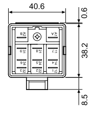
062.07 with relay
