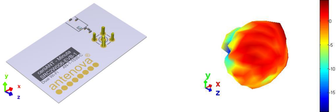
3D pattern at 5.46GHz Drag to rotate pattern and PCB by using Adobe Reader (Click to Activate)
