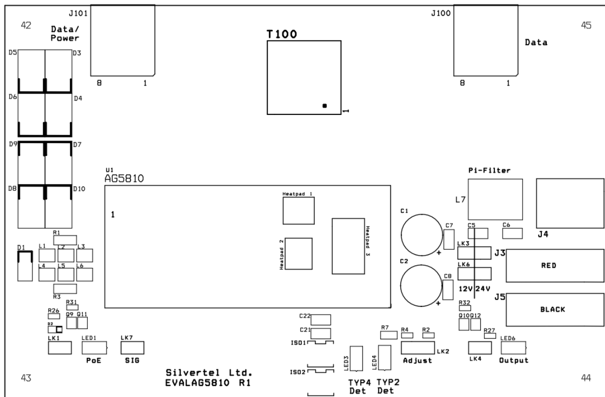
Figure 1: Board Layout
