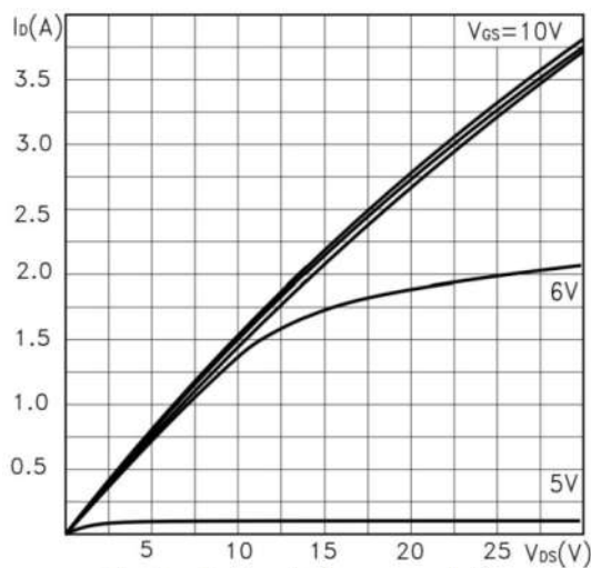
Fig.3 Output characteristics
