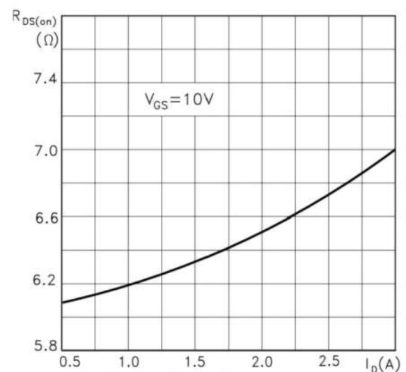
Fig.6 Static drain-source on resistance
