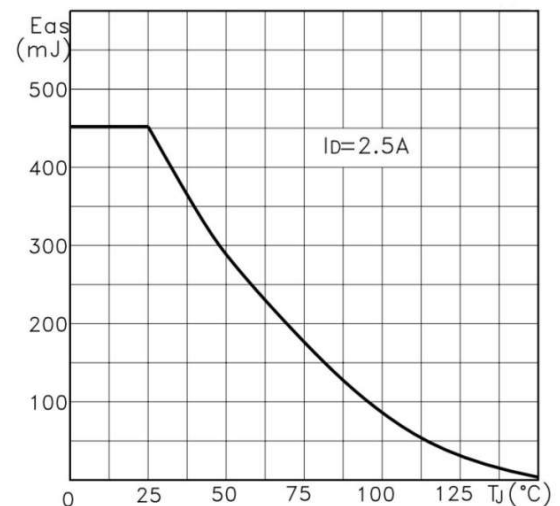
Fig.12 Maximum avalanche energy vs T_J
