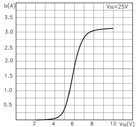
Fig.4 Transfer characteristics
