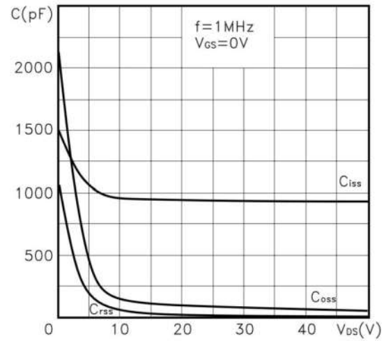
Fig.8 Capacitance variations
