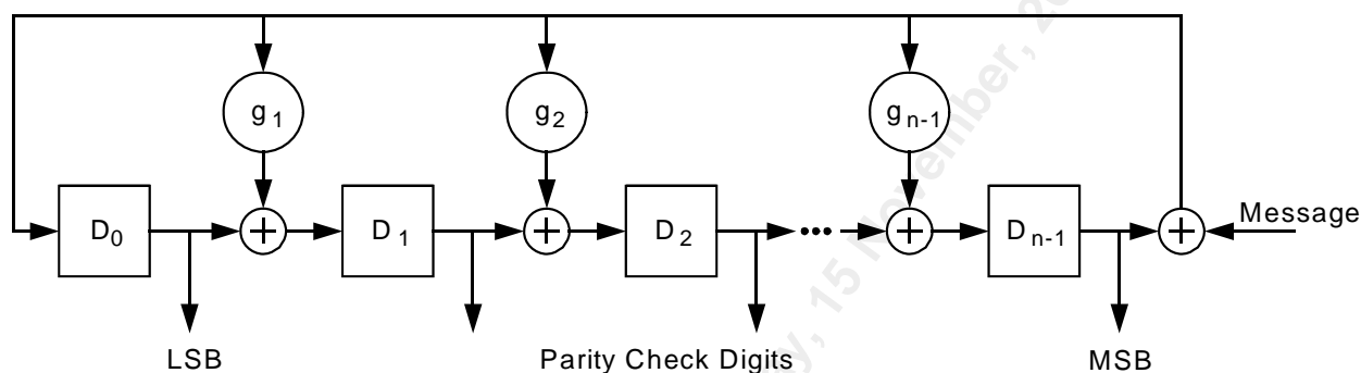
Figure 10: CRC Generator
