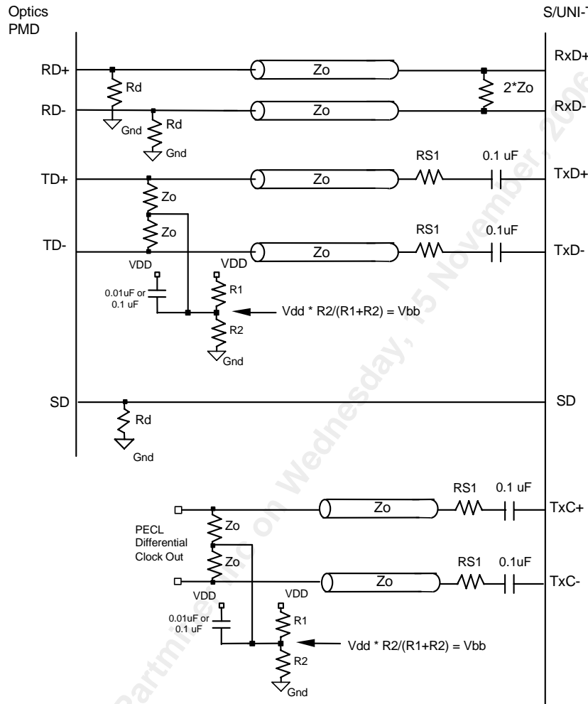
Figure 33: Interfacing to ECL or PECL
