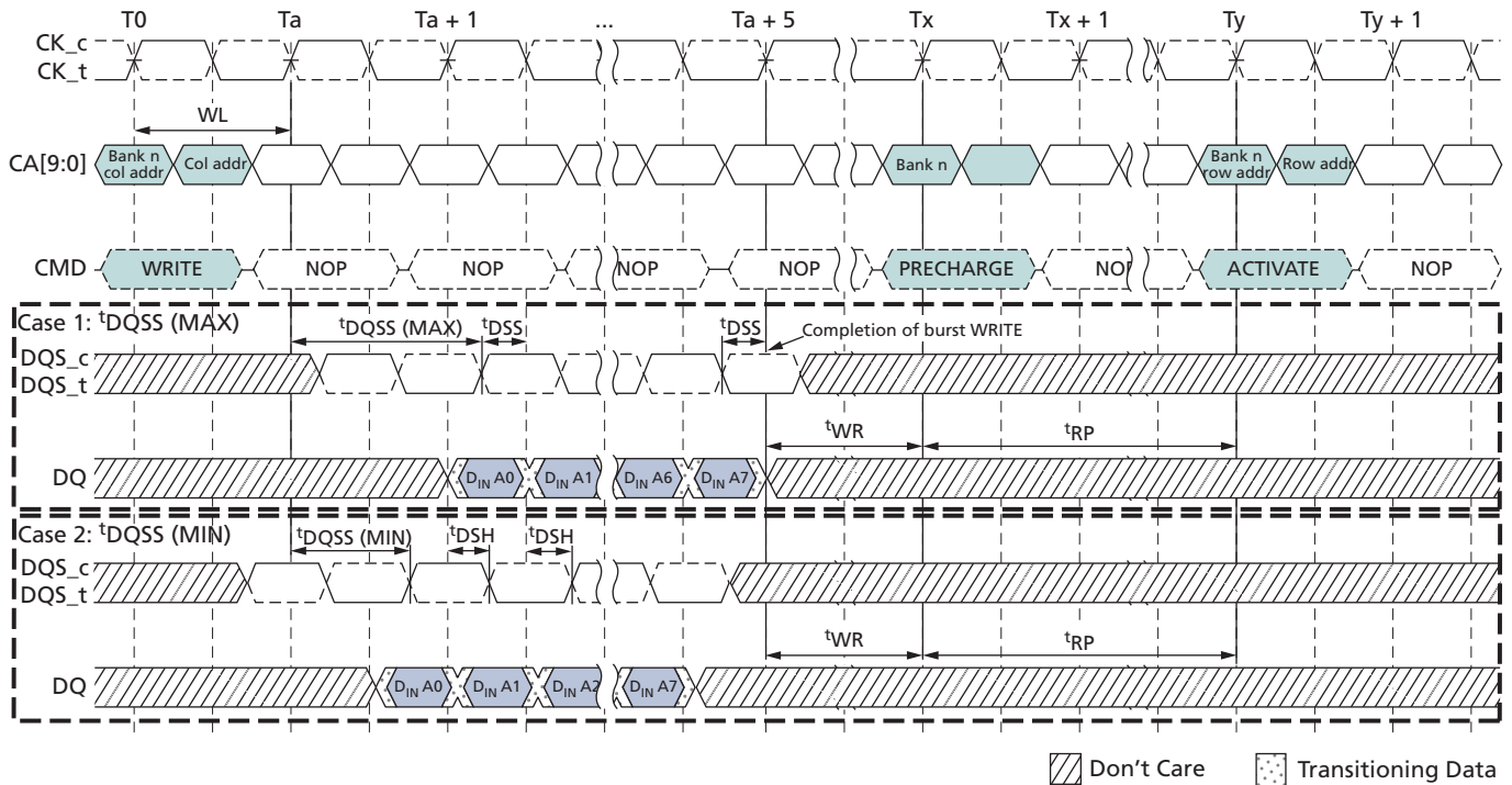
Figure 21: Burst WRITE
