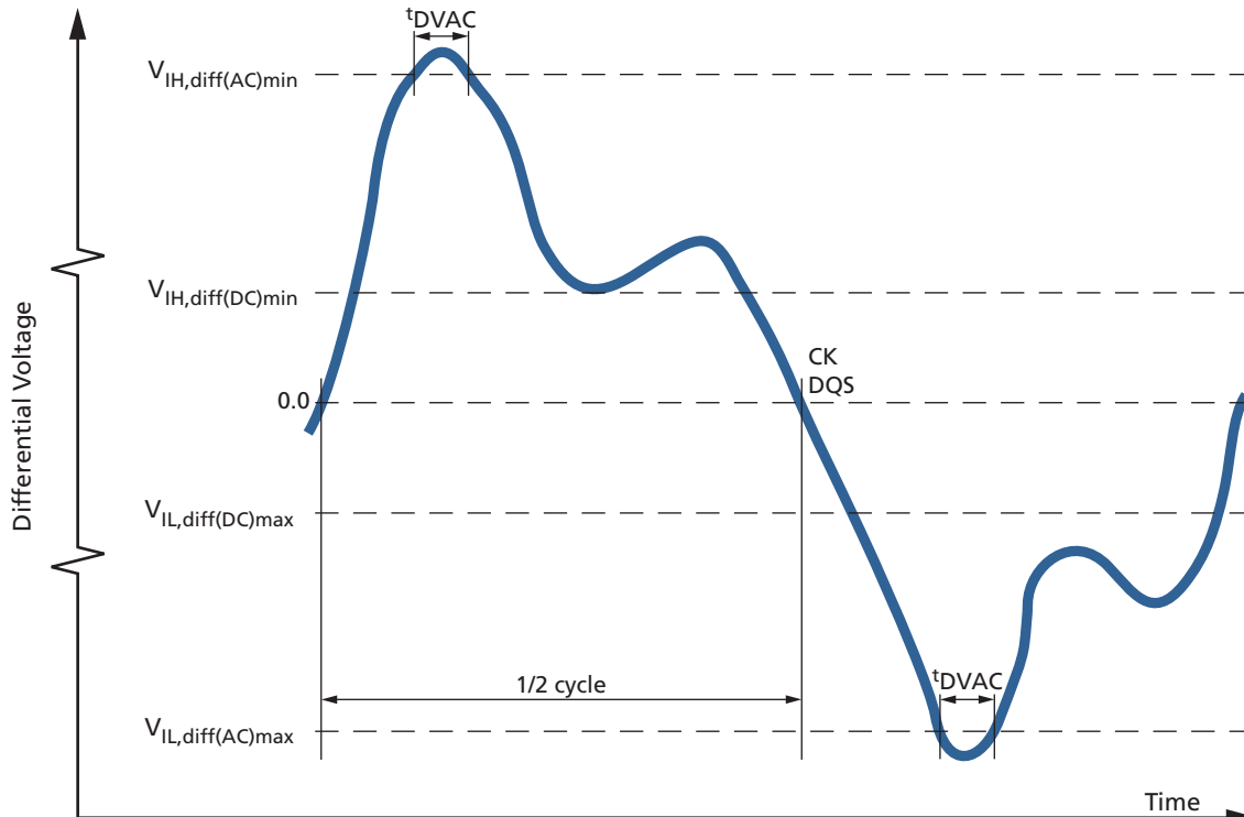
Figure 69: Differential AC Swing Time and t_{DVAC}
