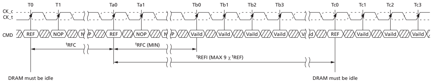
Figure 32: REFRESH Command Timing
