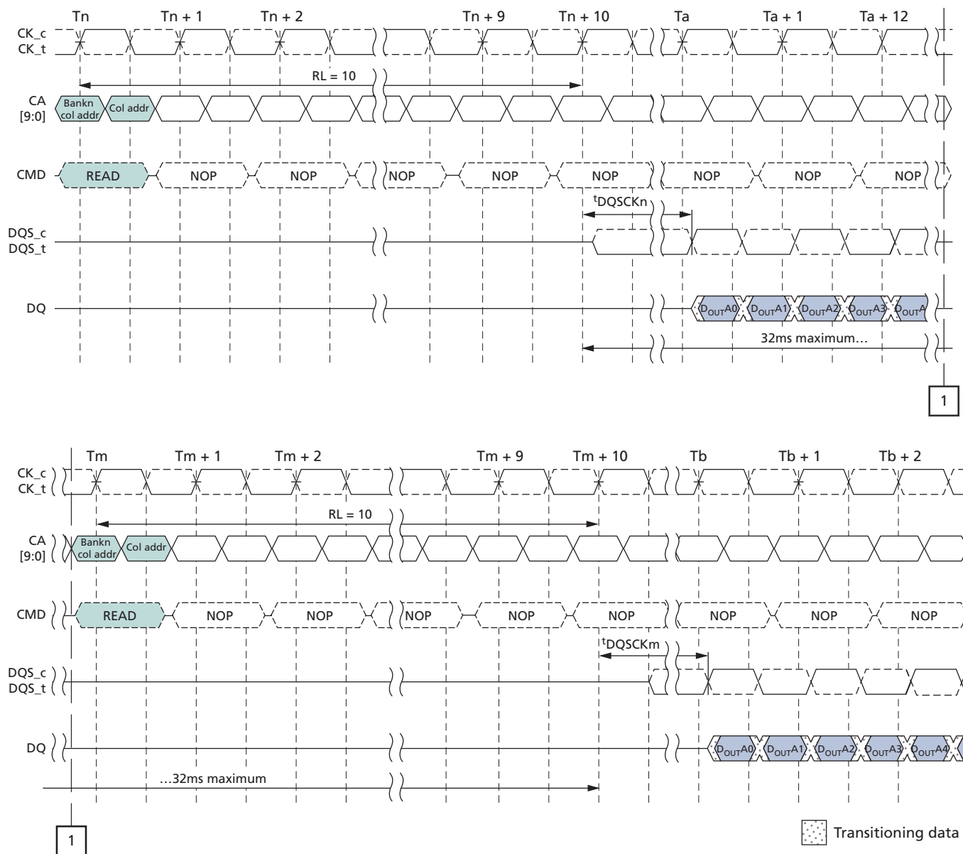
Figure 17: t_{DQSKDL} Timing
