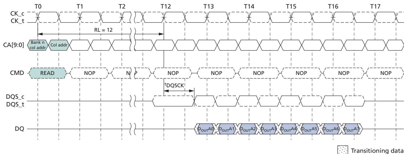
Figure 14: Burst READ – RL = 12, BL = 8, t_{DQSCK} < t_{CK}
