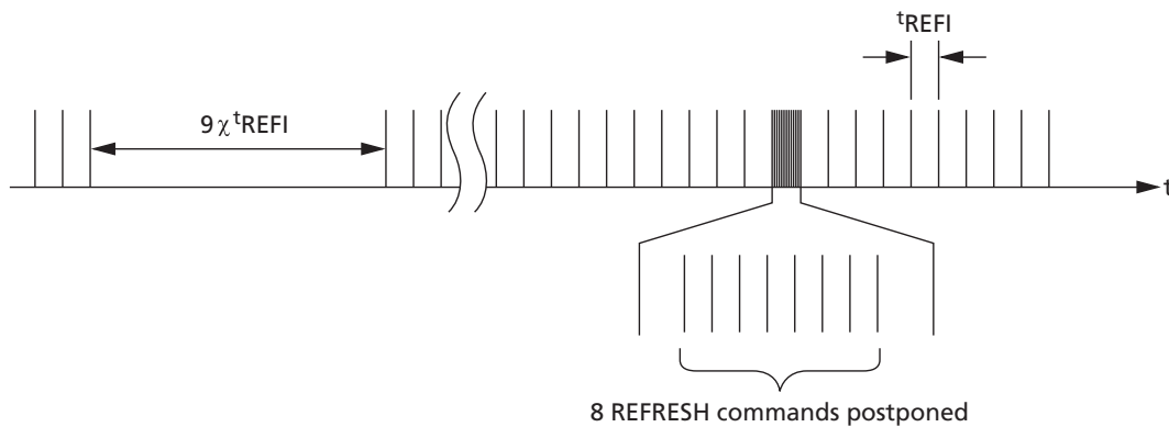
Figure 33: Postponing REFRESH Commands
