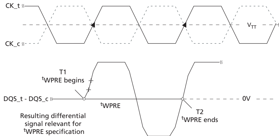
Figure 22: Method for Calculating tWPRES Transitions and Endpoints
