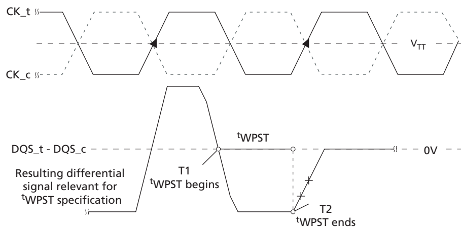
Figure 23: Method for Calculating t_{WPST} Transitions and Endpoints
