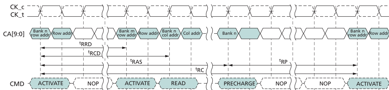
Figure 10: ACTIVATE Command
