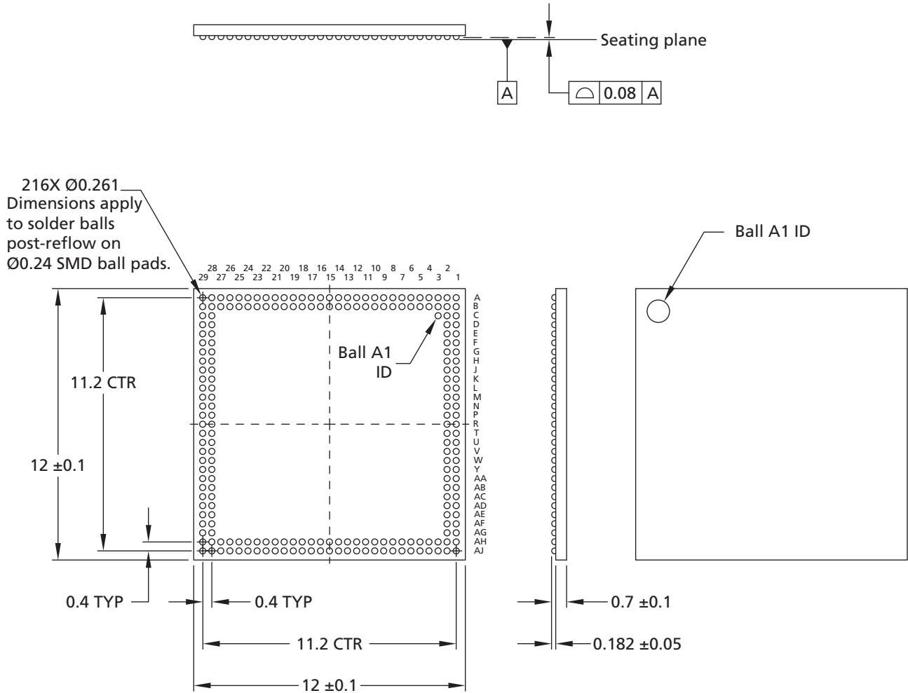
Figure 4: 216-Ball FBGA (12mm x 12mm)
