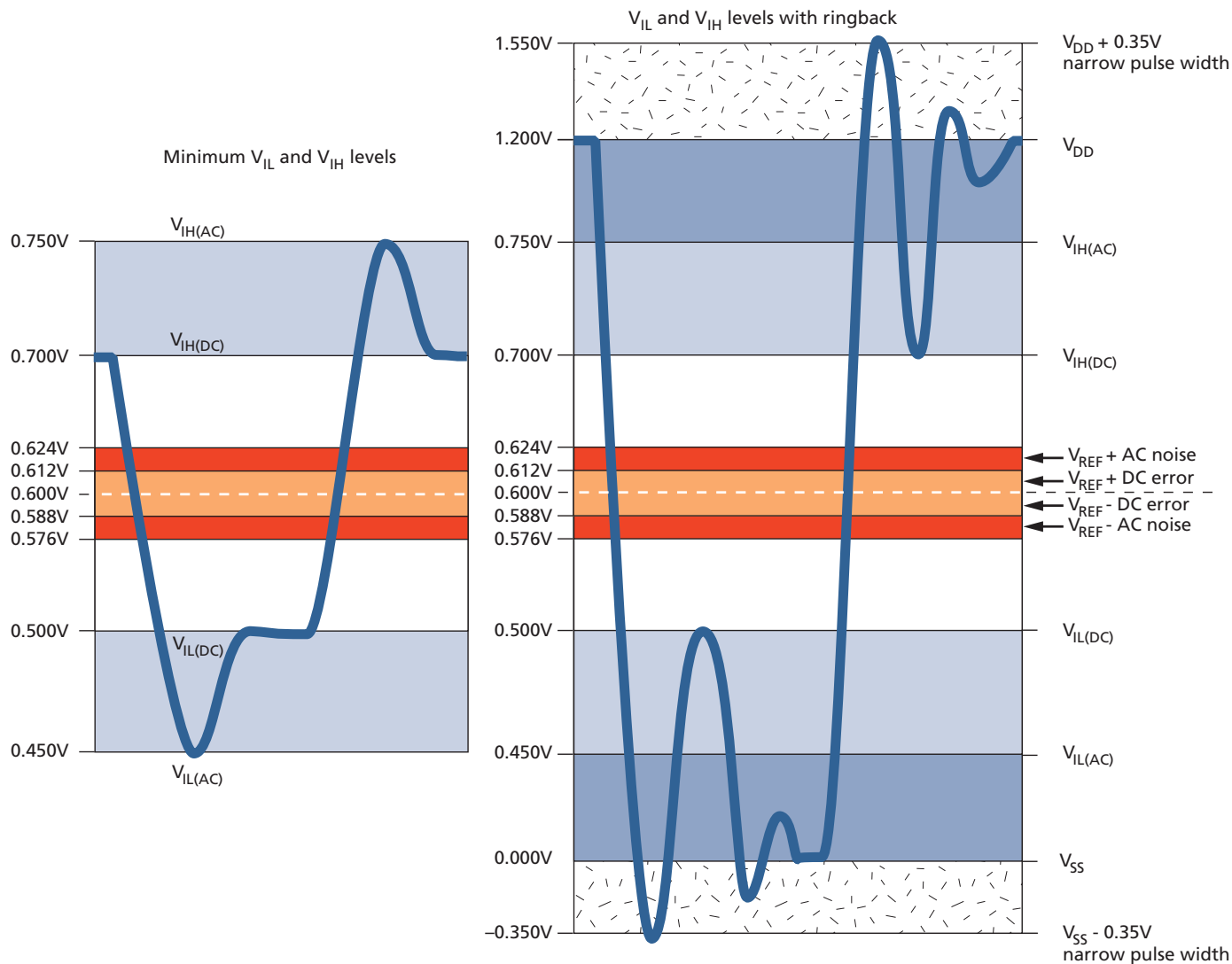
Figure 67: LPDDR3-1600 to LPDDR3-1333 Input Signal
