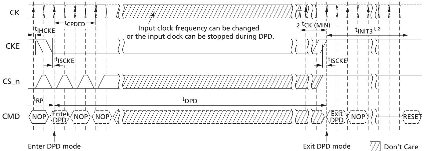
Figure 65: Deep Power-Down Entry and Exit Timing
