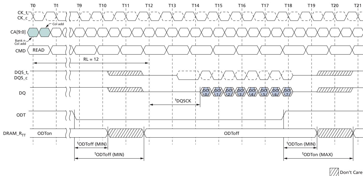
Figure 50: Asynchronous ODT Timing – RL = 12
