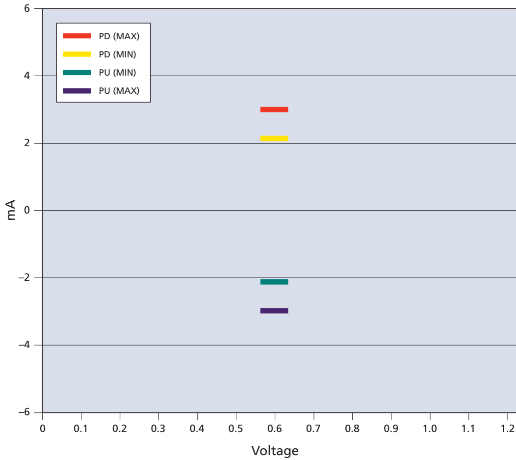
Figure 79: Output Impedance = 240\Omega , I-V Curves After Calibration
