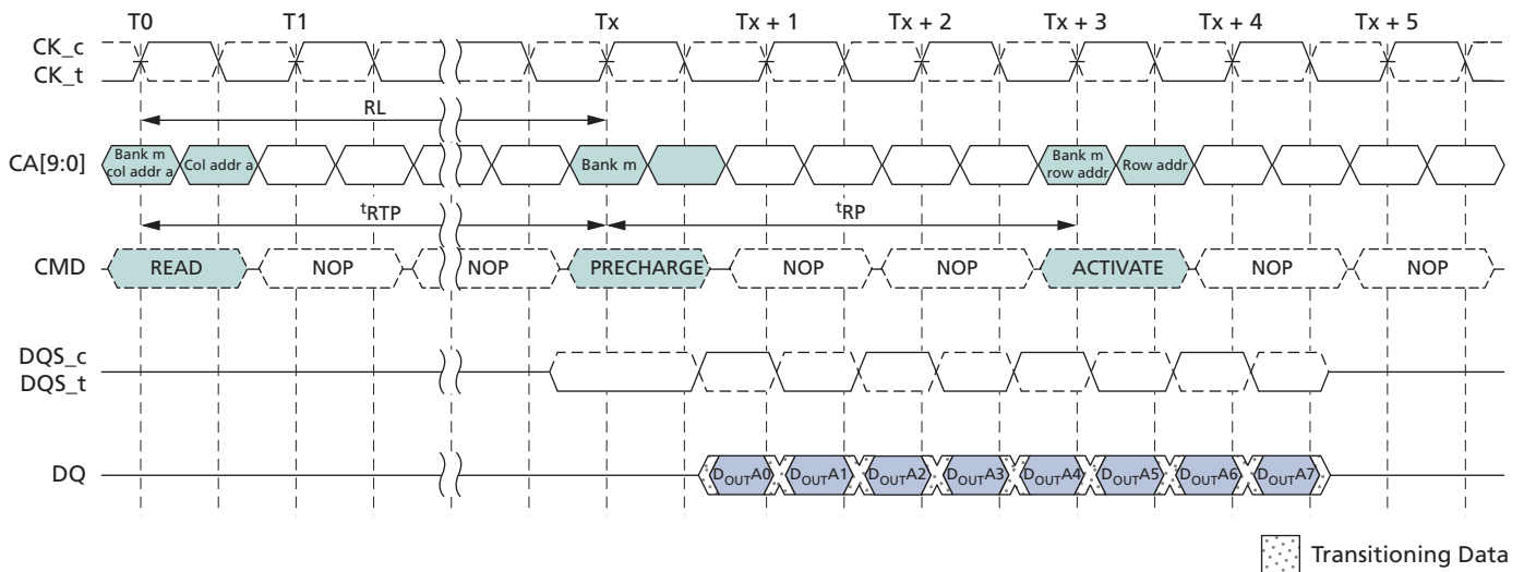
Figure 28: Burst READ Followed by PRECHARGE – BL = 8, RU(t_{RTP}(\text{MIN})/t_{CK}) = 2
