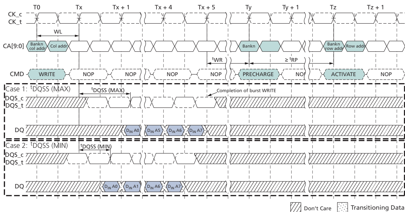
Figure 29: Burst WRITE Followed by PRECHARGE – BL = 8
