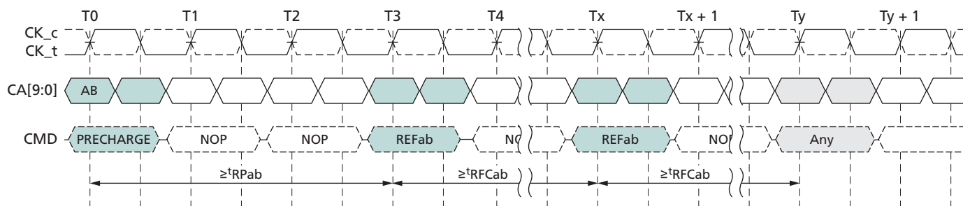
Figure 35: All-Bank REFRESH Operation
