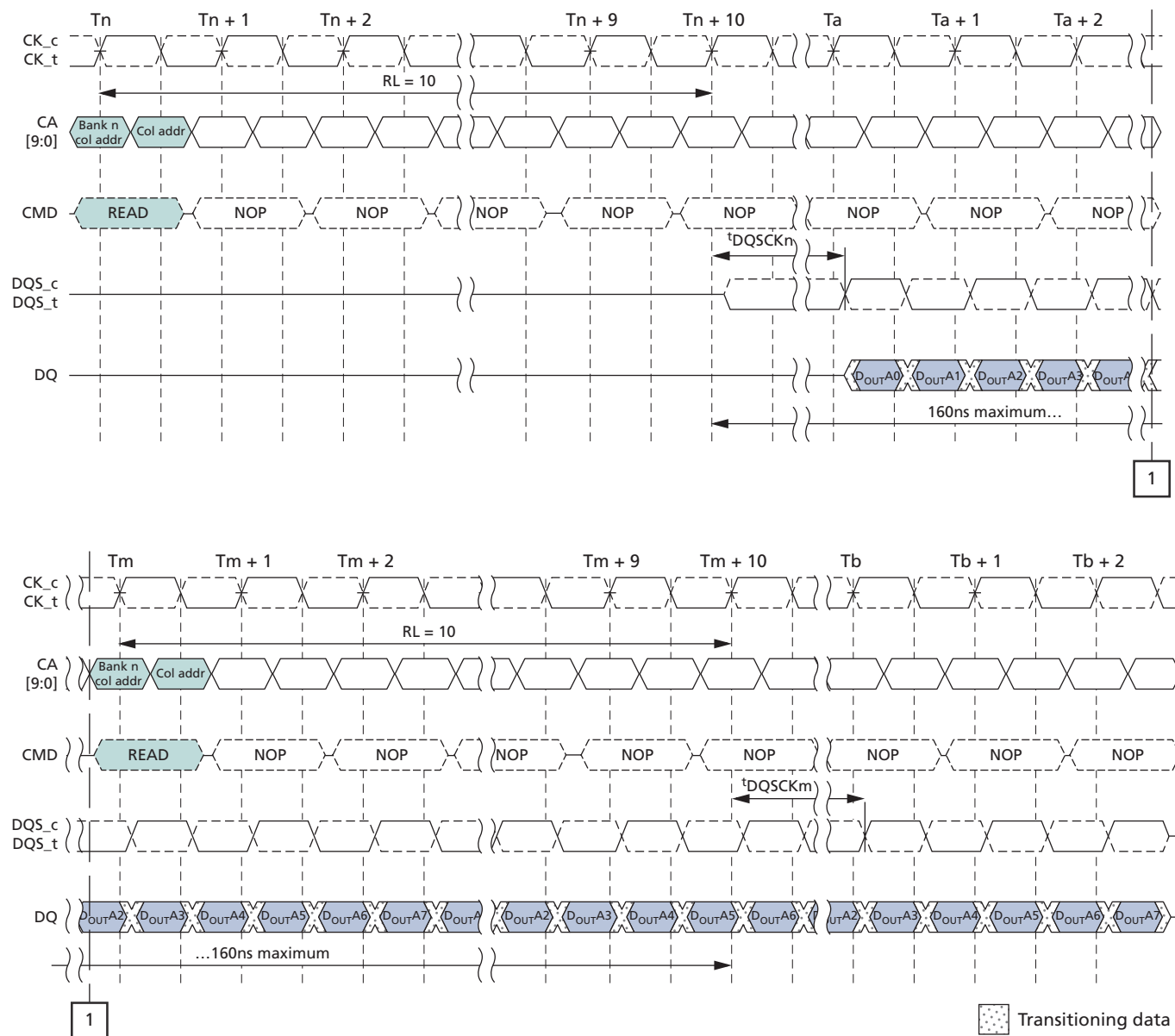
Figure 19: t_{DQSKDS} Timing
