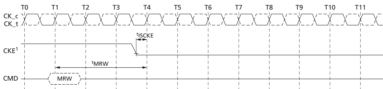
Figure 64: MRW Command to Power-Down Entry
