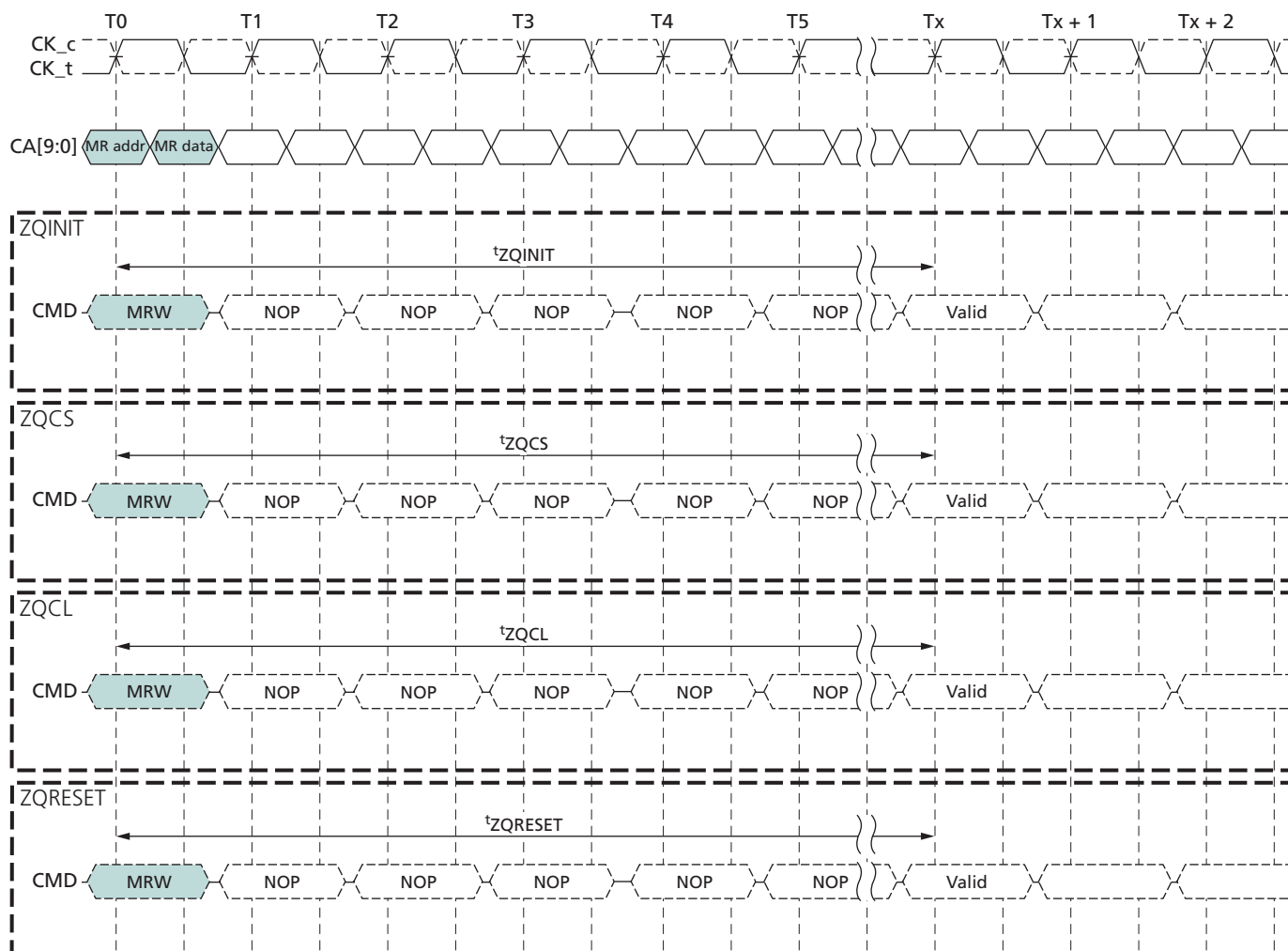
Figure 46: ZQ Timings
