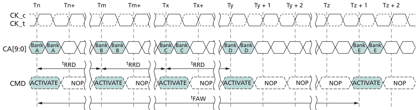
Figure 11: t_{FAW} Timing
