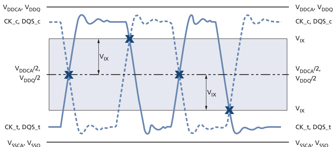
Figure 71: V_{IX} Definition
