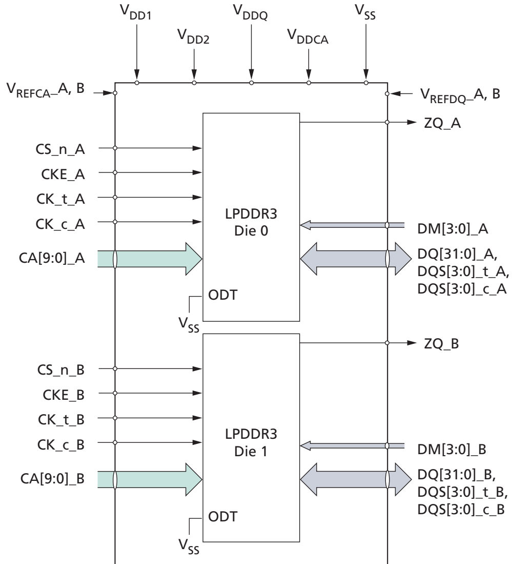
Figure 3: Dual-Die, Dual-Channel Package Block Diagram
