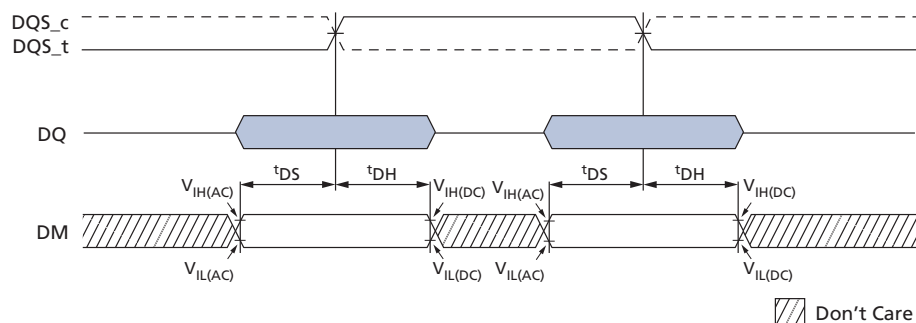
Figure 26: Data Mask Timing
