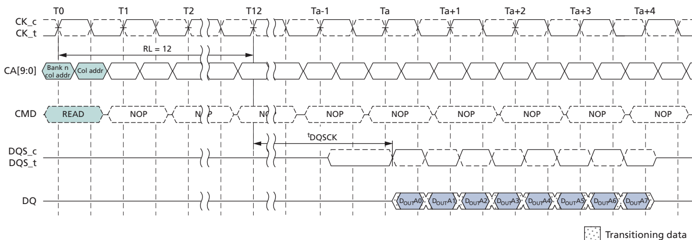
Figure 13: Burst READ – RL = 12, BL = 8, t_{DQSCK} > t_{CK}
