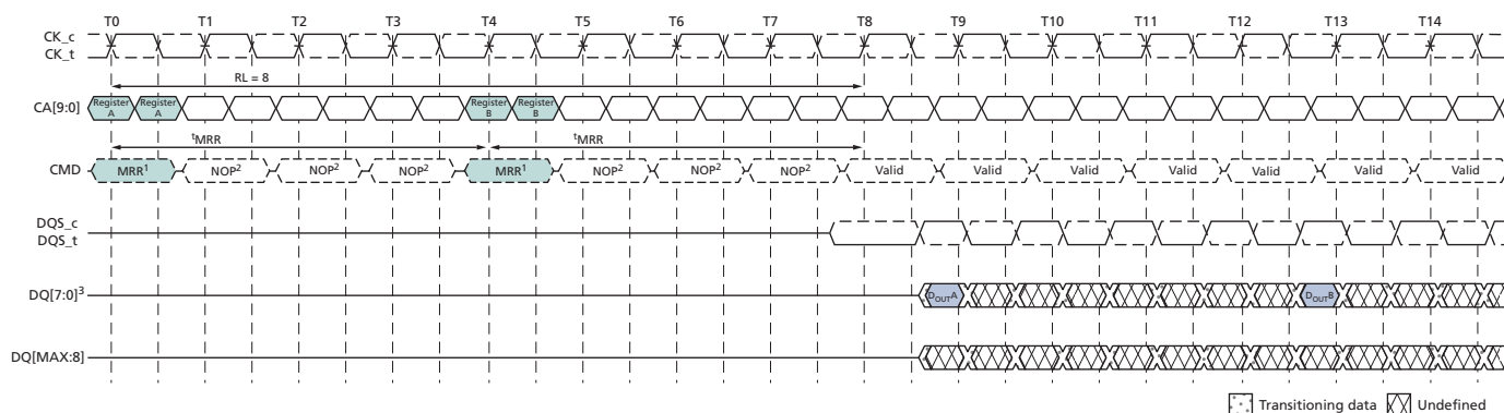
Figure 38: MRR Timing
