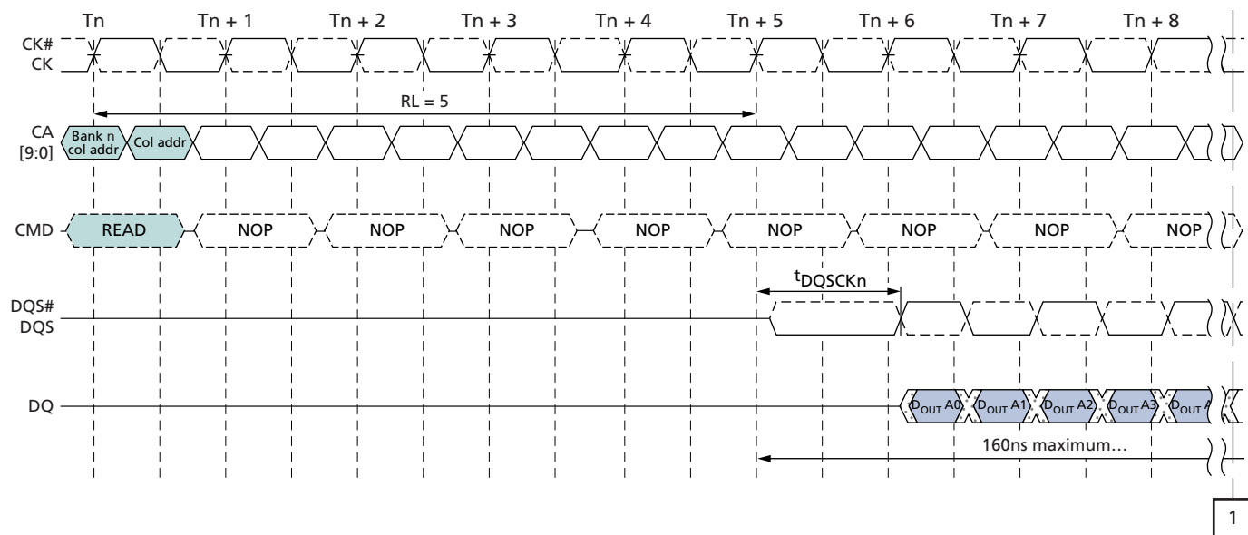
Figure 18: t_{DQSKDS} Timing
