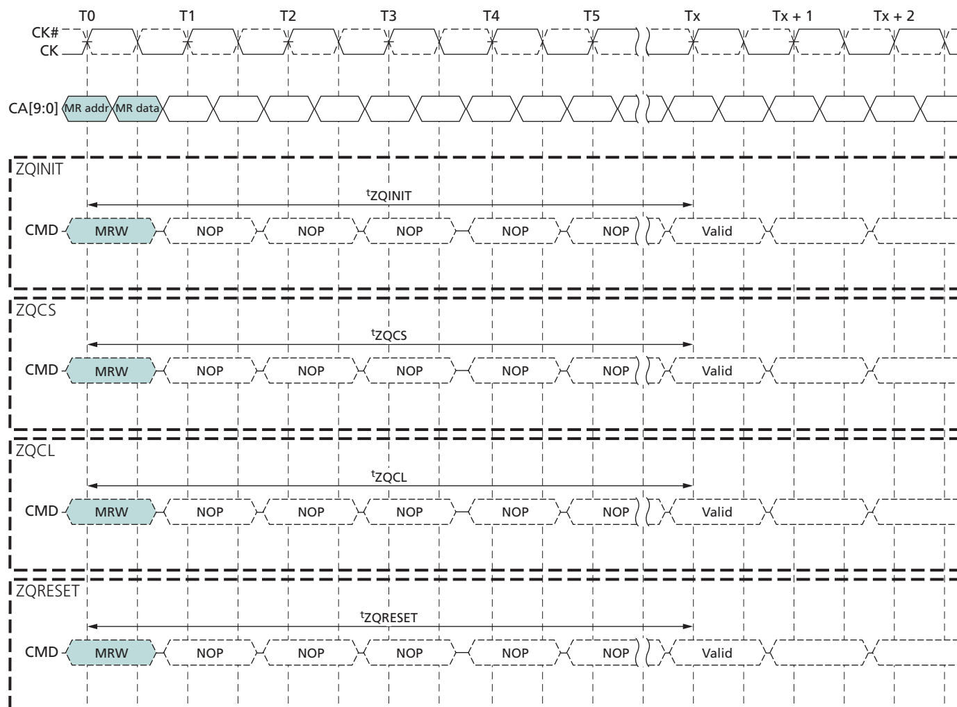
Figure 50: ZQ Timings
