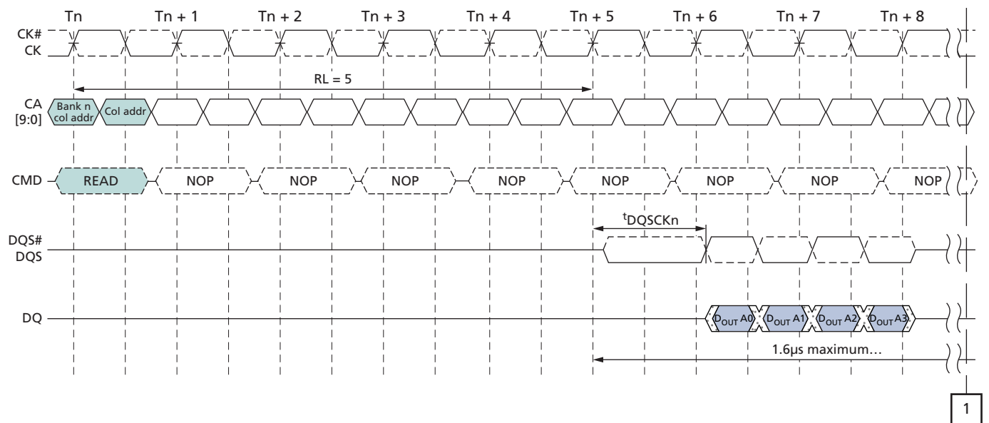
Figure 17: t_{DQSCDM} Timing
