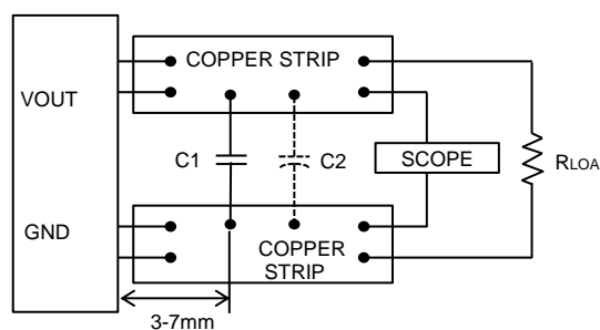
C1=220 \mu\text{F} x 2 or 100 \mu\text{F} x 4 CERAMIC C2=OPEN Figure: Measuring Output Ripple and Noise
