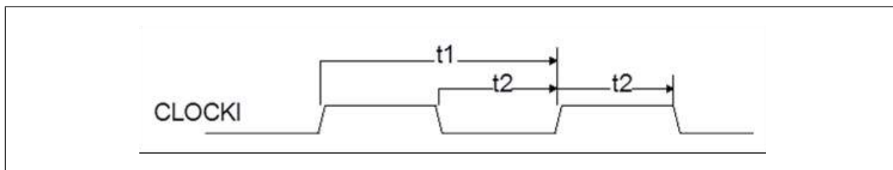
FIGURE 22-2: INPUT CLOCK TIMING
