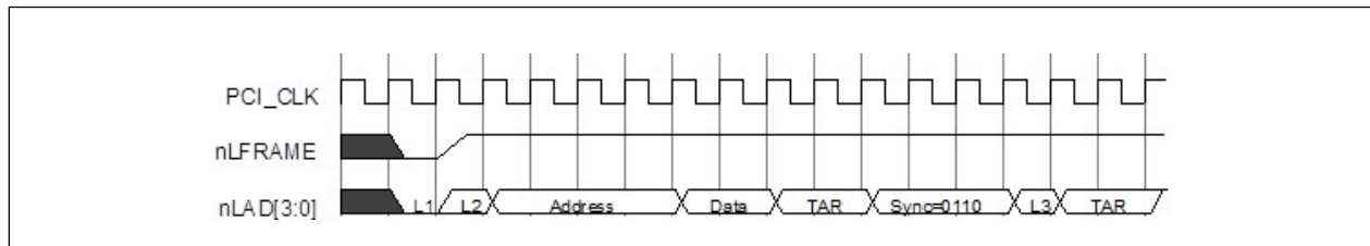
FIGURE 22-7: I/O WRITE
