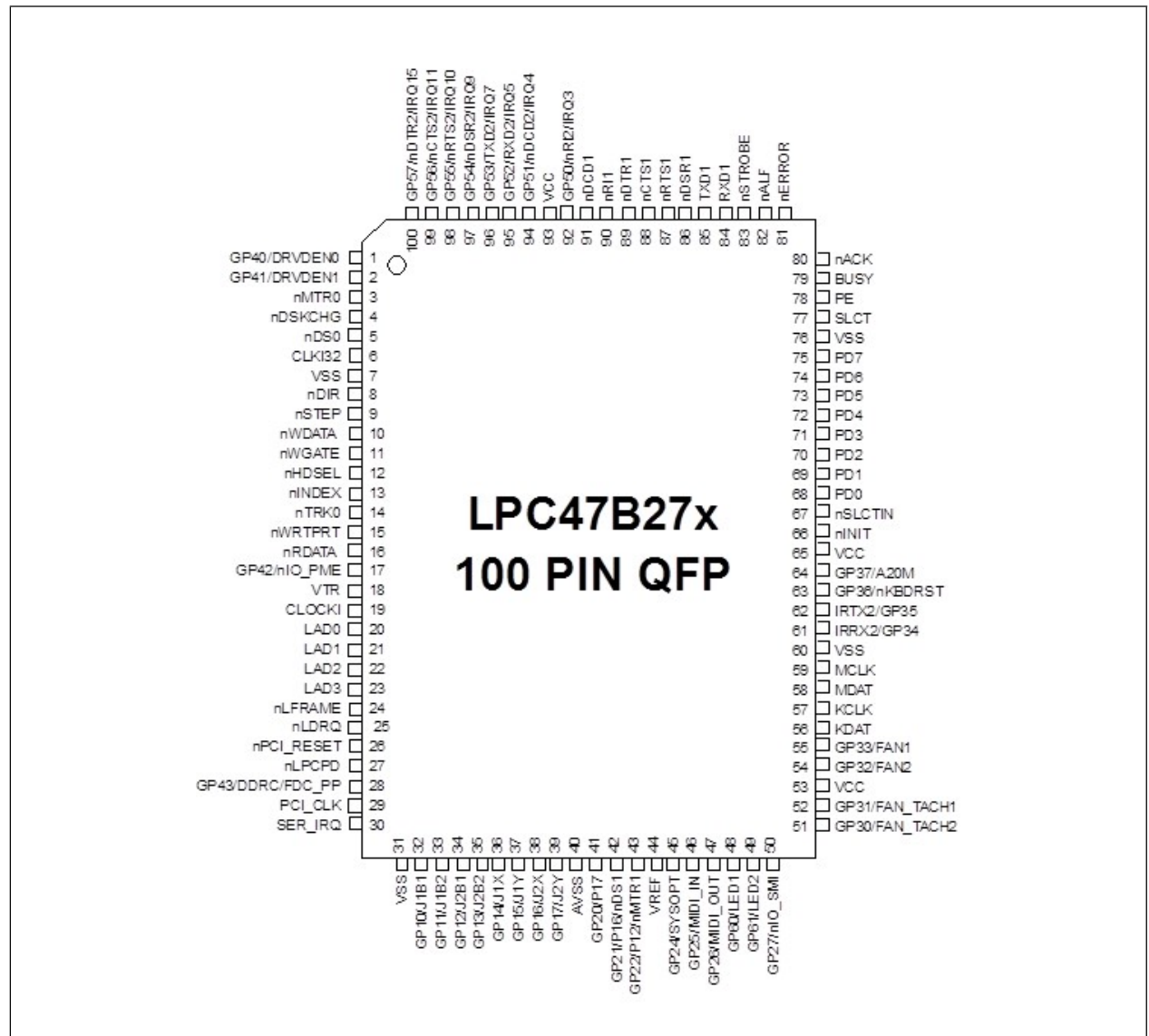
FIGURE 2-1: LPC47B27X 100 PIN QFP
