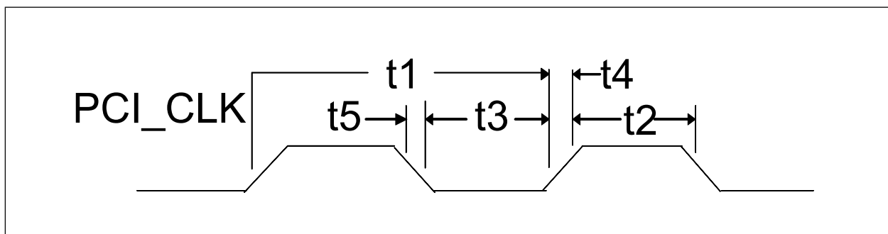
FIGURE 22-3: PCI CLOCK TIMING
