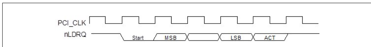
FIGURE 22-9: DMA REQUEST ASSERTION THROUGH NLDRQ
