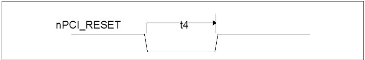
FIGURE 22-4: RESET TIMING
