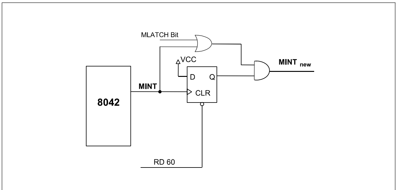
FIGURE 13-2: MOUSE LATCH
