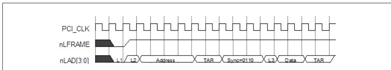
FIGURE 22-8: I/O READ
