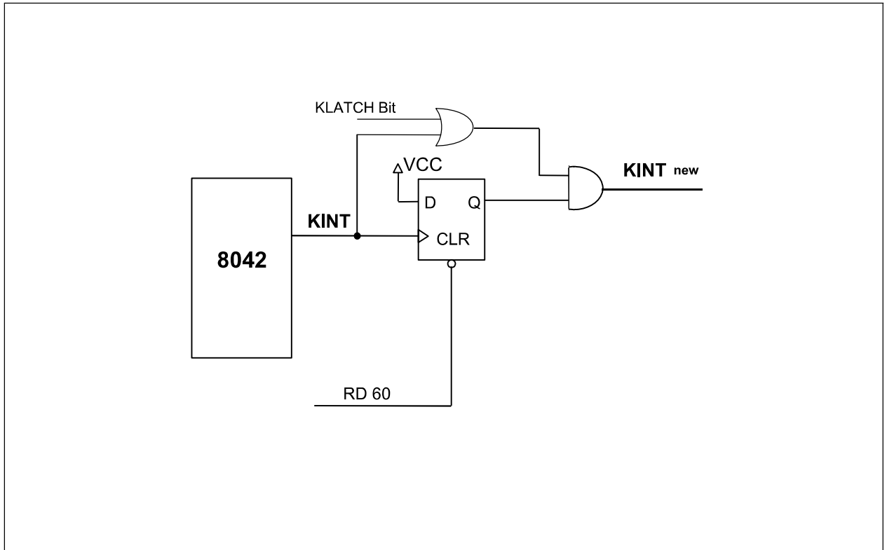
FIGURE 13-1: KEYBOARD LATCH
