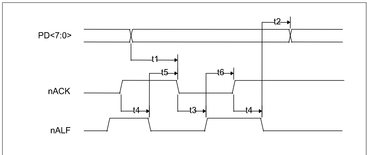
FIGURE 22-19: ECP PARALLEL PORT REVERSE TIMING
