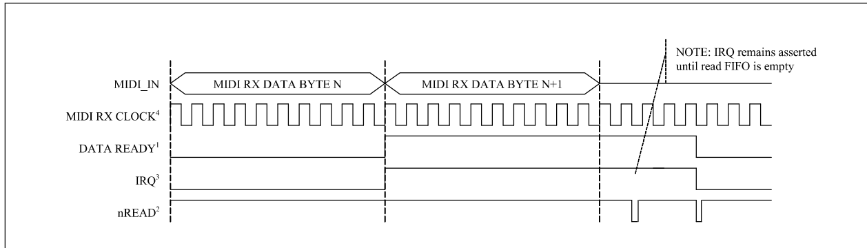
FIGURE 9-2: MPU-401 INTERRUPT
