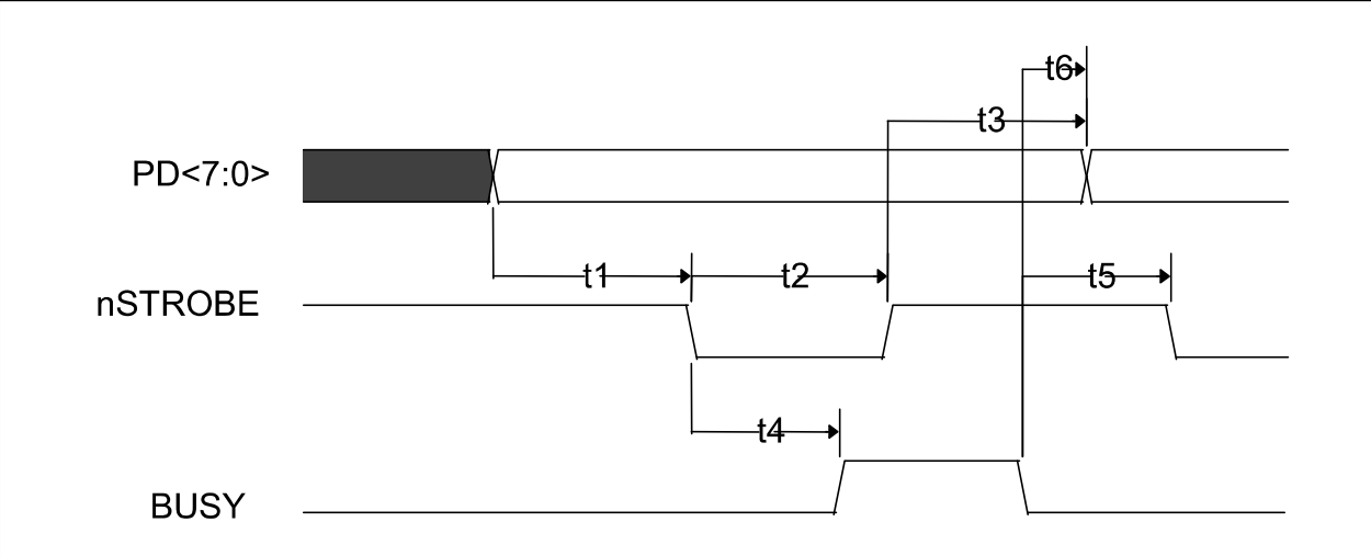
FIGURE 22-17: PARALLEL PORT FIFO TIMING
