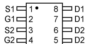
pin assignment
