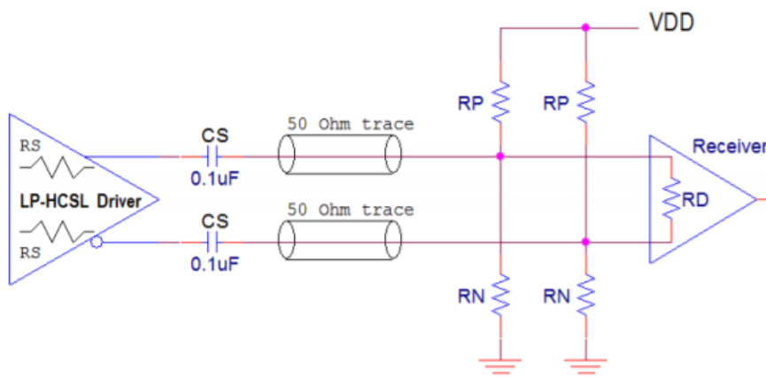
Figure 13. AC-Coupling Termination
