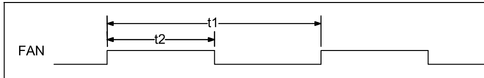
FIGURE 32 – FAN OUTPUT TIMING
