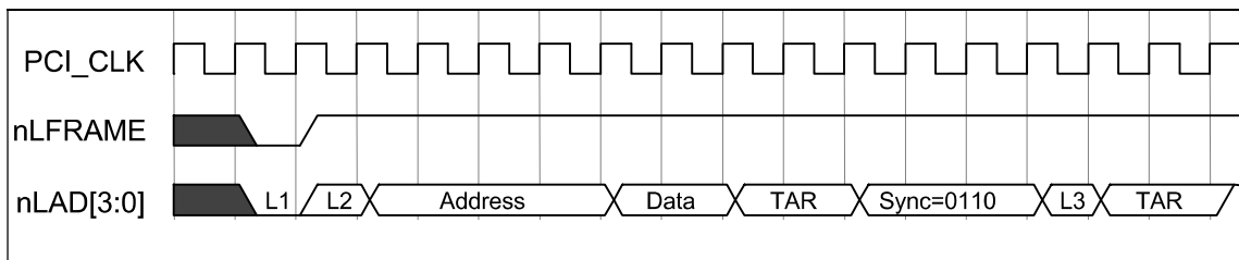
FIGURE 11 – I/O WRITE
