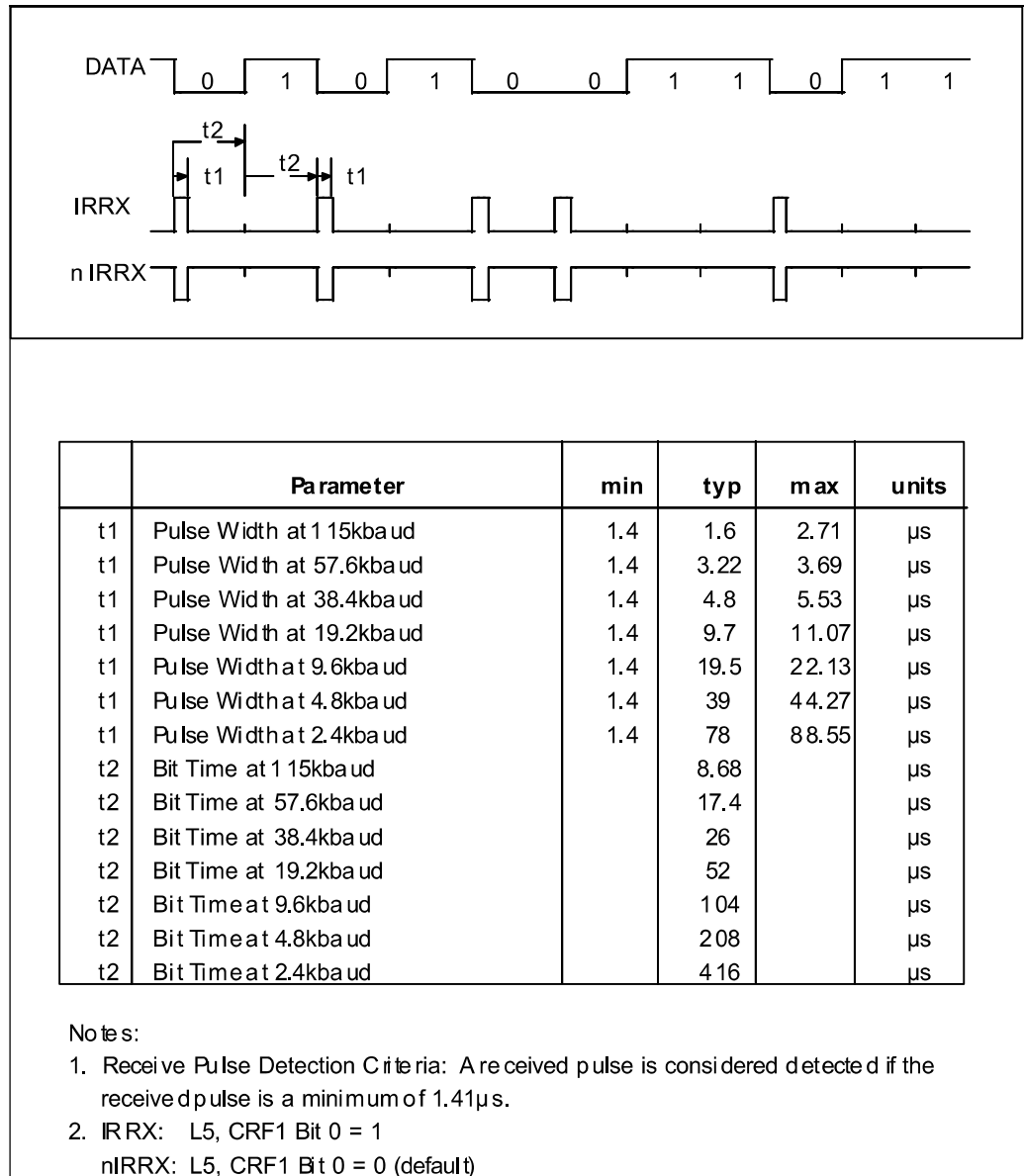
FIGURE 24 - IrDA RECEIVE TIMING
