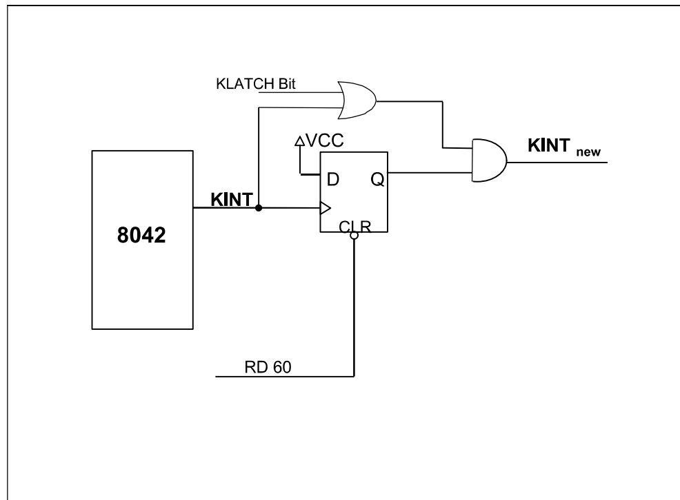
FIGURE 3 - KEYBOARD LATCH
