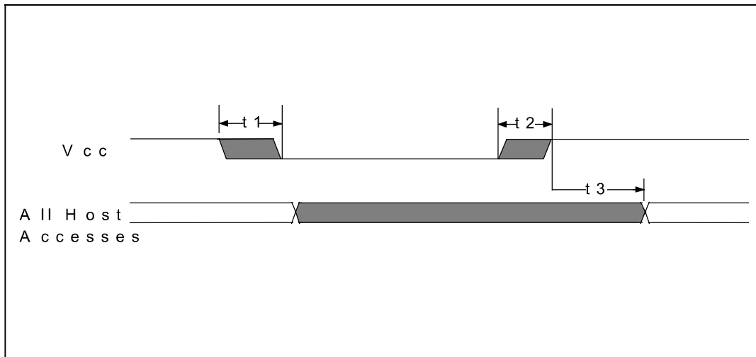
FIGURE 7 - POWER-UP TIMING
