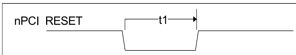
FIGURE 8C - RESET TIMING
