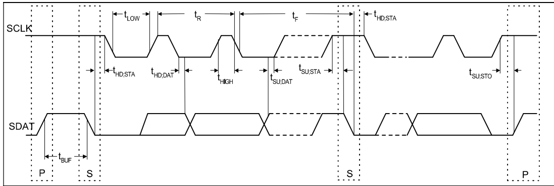
FIGURE 28 - SMBUS TIMING
