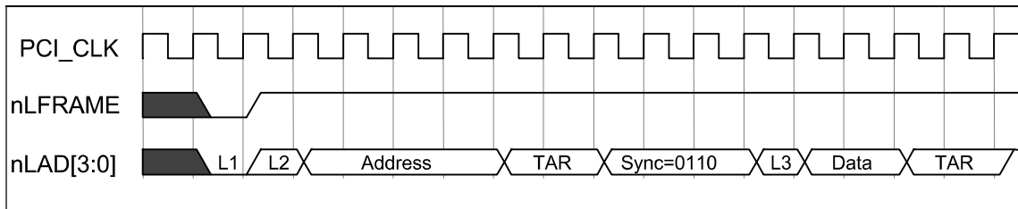
FIGURE 12 – I/O READ
