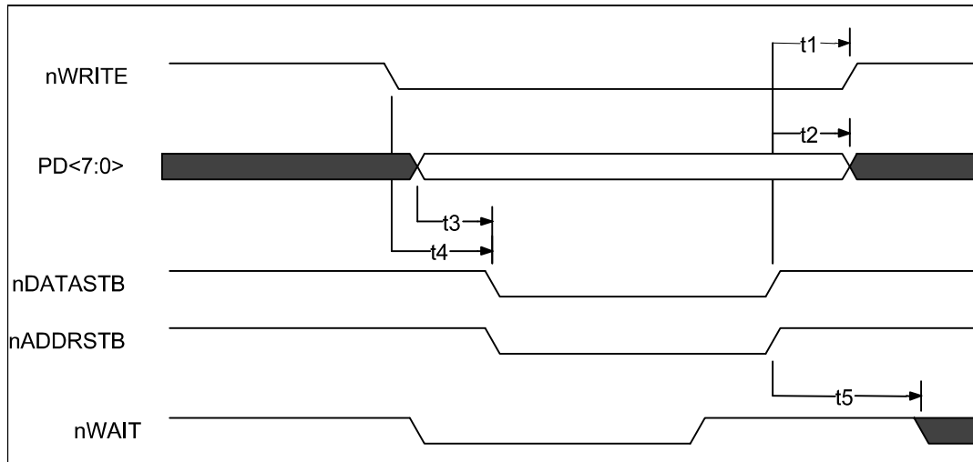
FIGURE 19 – EPP 1.7 DATA OR ADDRESS WRITE CYCLE
