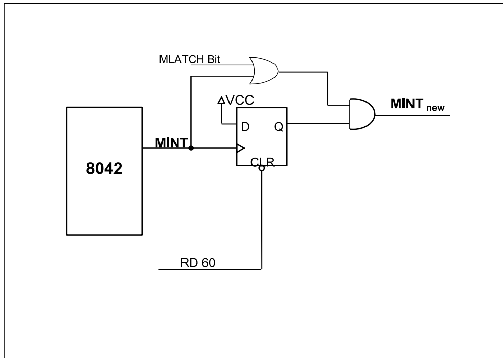
FIGURE 4 – MOUSE LATCH
