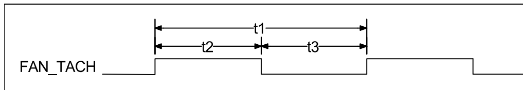
FIGURE 33 – FAN TACHOMETER INPUT TIMING
