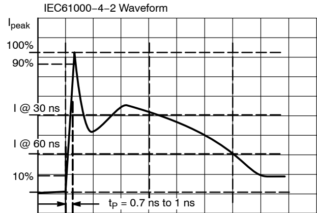
Figure 4. IEC61000-4-2 Spec
