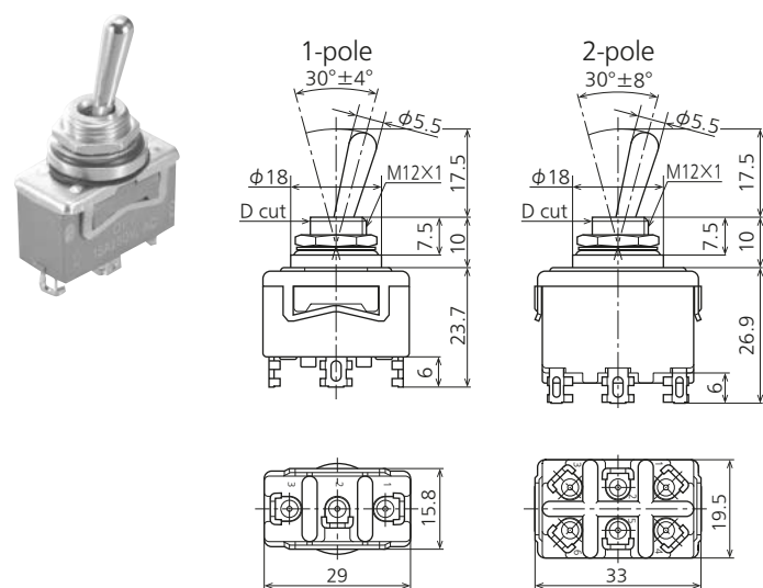
External dimensions
