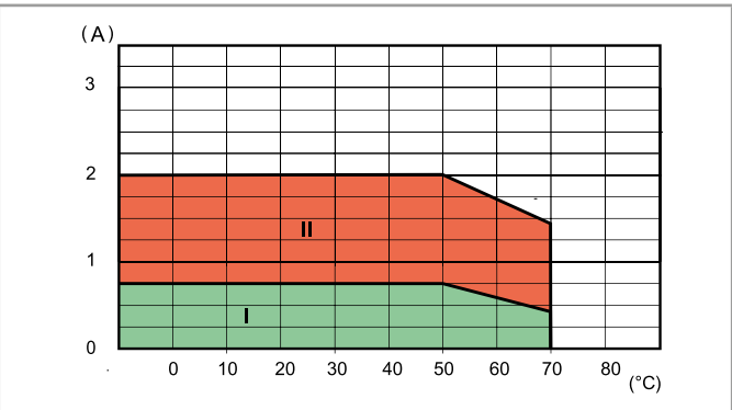
L 39-2 - Output AC current v ambient temperature
