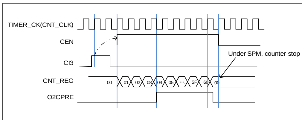
图 17-19. 单脉冲模式, TIMERx_CHxCV = 0x04 , TIMERx_CAR=0x60
