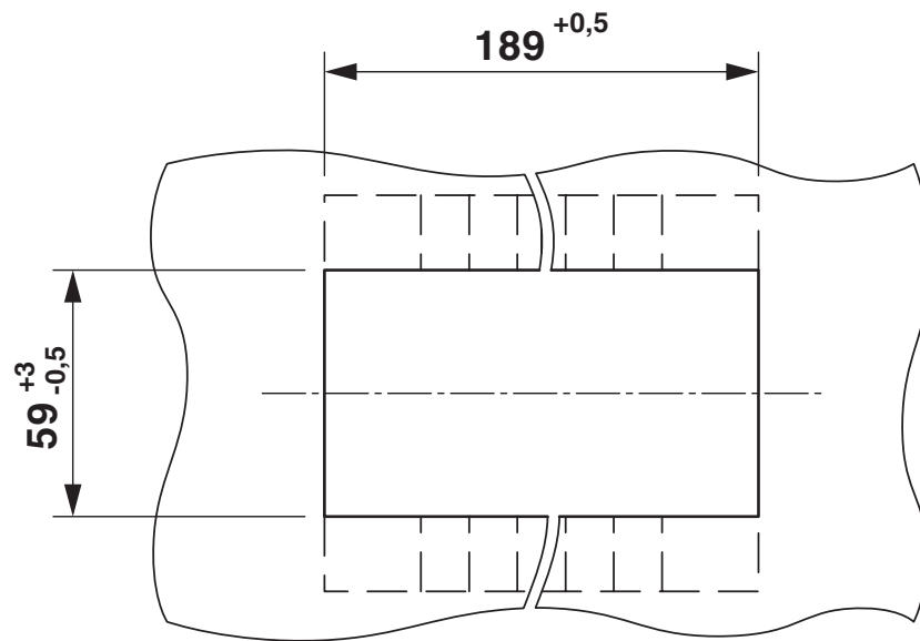
Dimensional drawing
