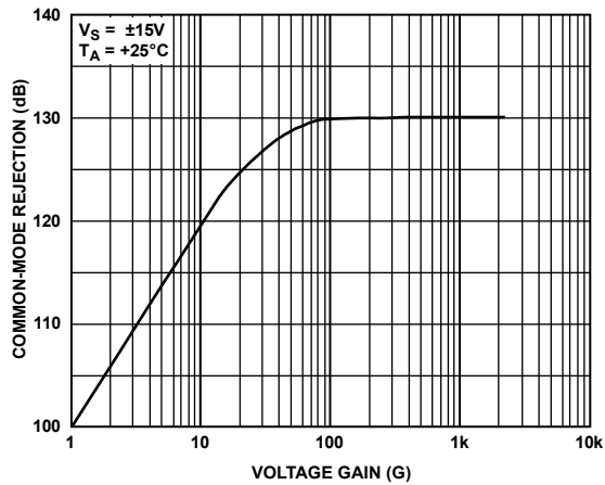
Figure 12. Common-Mode Rejection vs. Voltage Gain
