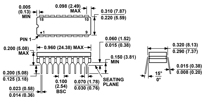
Figure 51. 18-Lead Ceramic Dual In-Line Package [CERDIP] (O-18)
