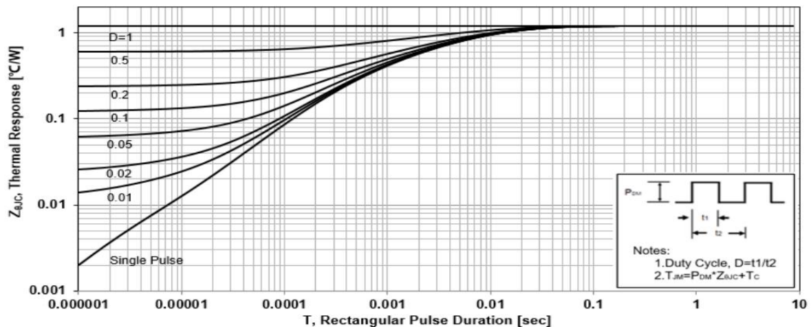
Figure 5. Transient Thermal Impedance
