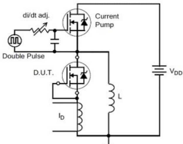
Figure 18. Diode Reverse Recovery Test Circuit
