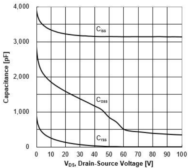
Figure 12. Capacitance Characteristics
