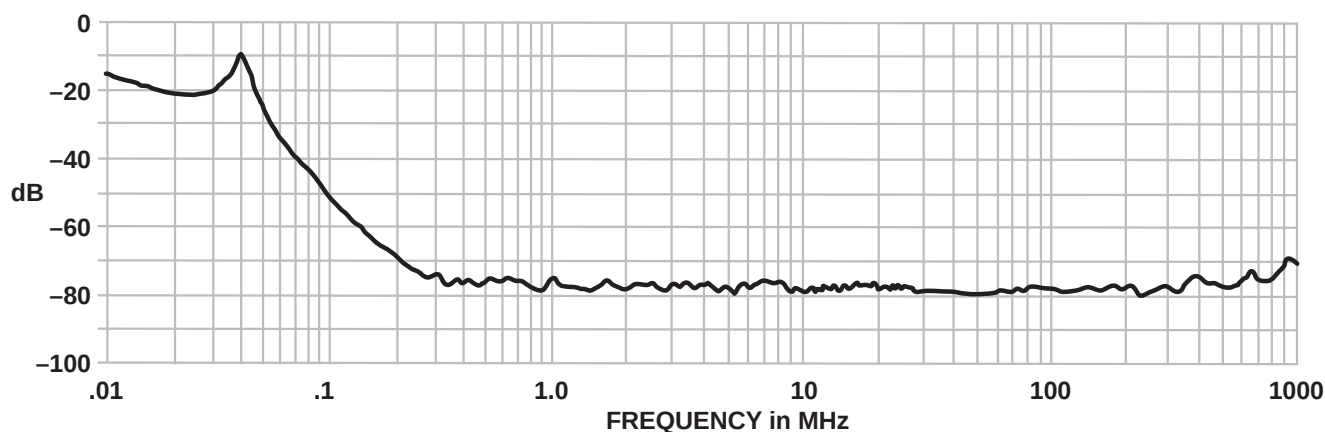
F5600 SERIES TYPICAL COMMON MODE INSERTION LOSS — dB (50 OHM CIRCUIT)
