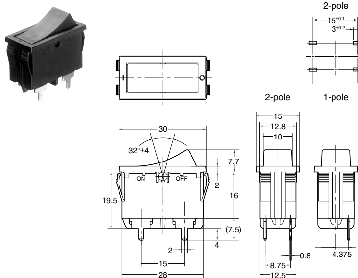
External dimensions
