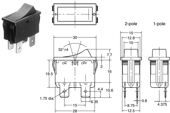
External dimensions
