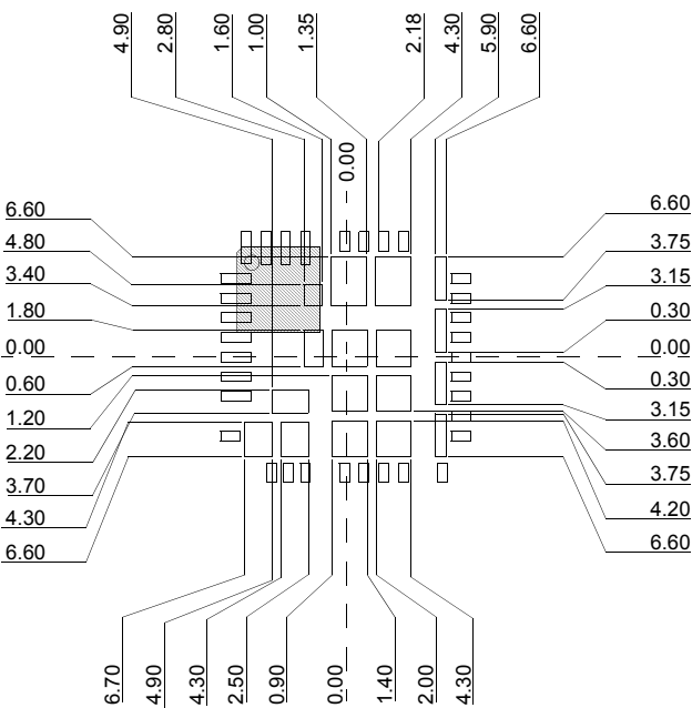
STENCIL PATTERN WITH SQUARE PADS-1
