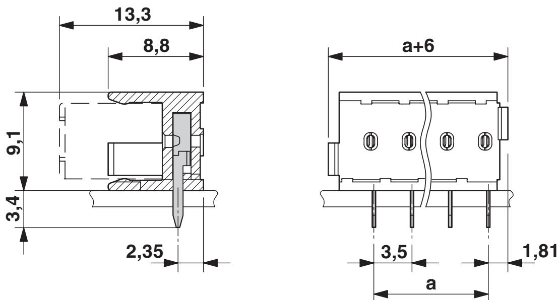
Dimensional drawing
