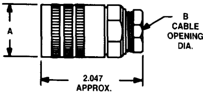
Cable Plug
