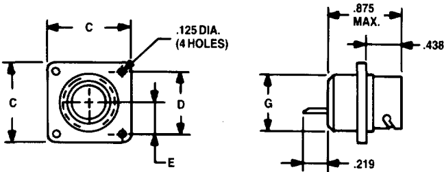
Panel Receptacle
