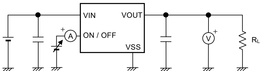
Figure 10 Test Circuit 4
