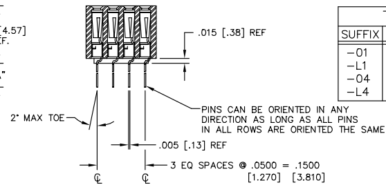
SECT "B-B"
