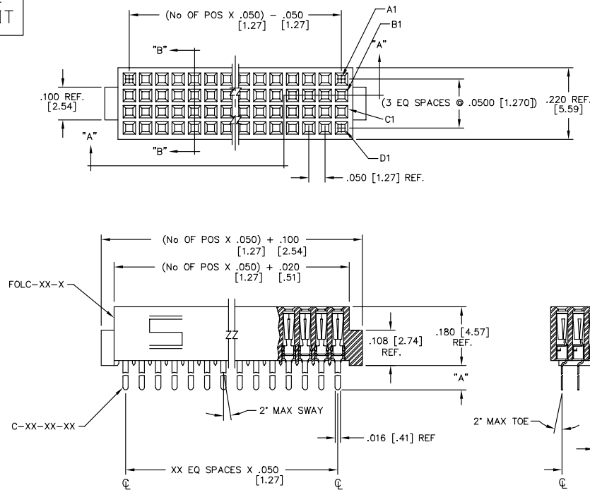
SECT "A-A"
