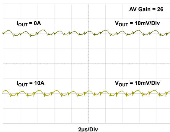
Figure 10. Output Ripple at 5V_{IN} and 1.8V_{OUT}
