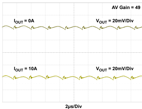
Figure 12. Output Ripple at 12V_{IN} and 1V_{OUT}
