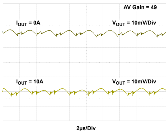
Figure 8. Output Ripple at 5V_{IN} and 1V_{OUT}
