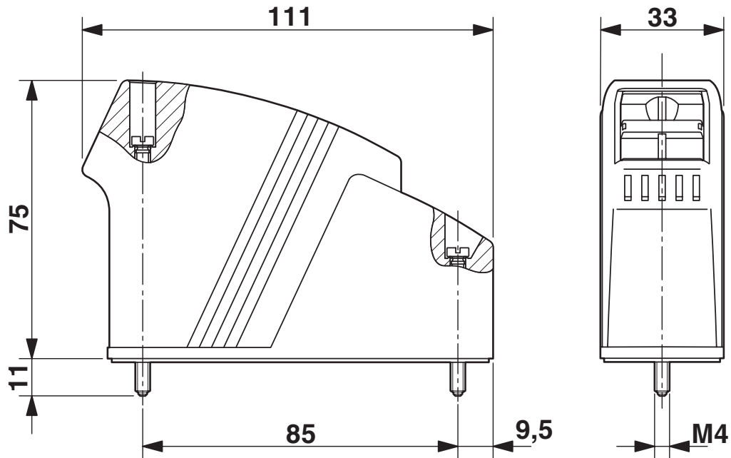
Dimensional drawing
